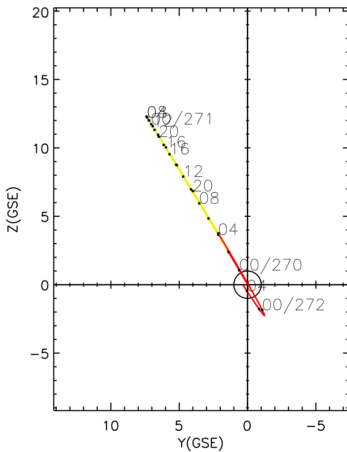
CLUSTER 2 orbit 2023 269 (09/26) 22:26 UT to 2023 272 (09/29) 04:36 UT
