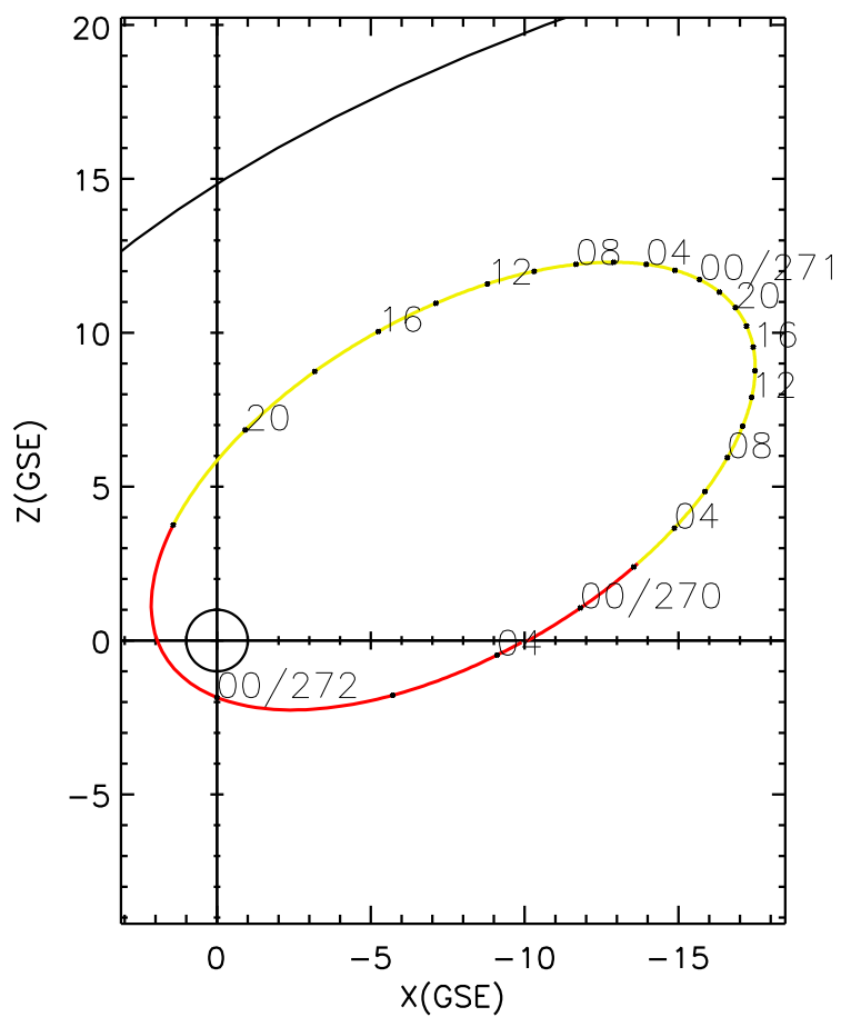
CLUSTER 2 orbit 2023 269 (09/26) 22:26 UT to 2023 272 (09/29) 04:36 UT
