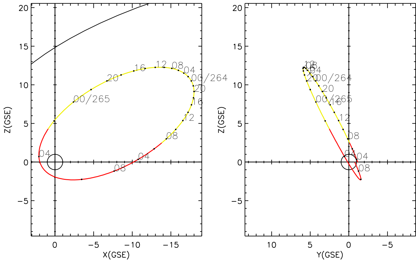
CLUSTER 2 orbit 2023 263 (09/20) 03:26 UT to 2023 265 (09/22) 09:41 UT
