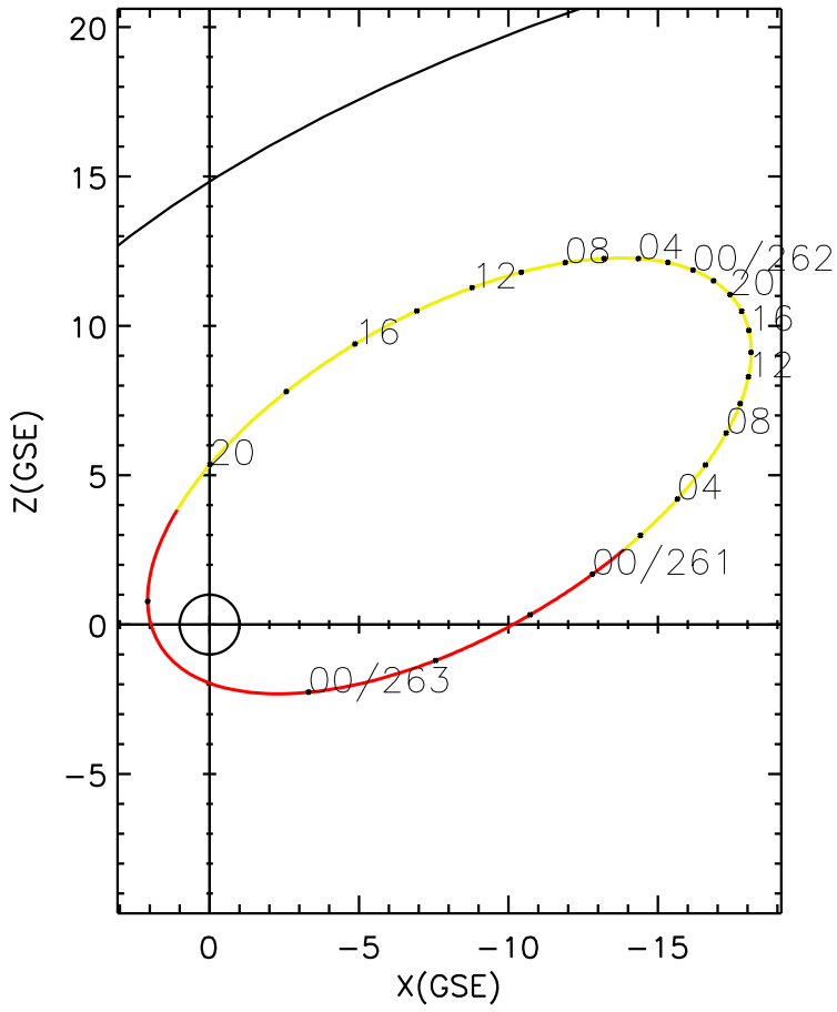
CLUSTER 2 orbit 2023 260 (09/17) 21:26 UT to 2023 263 (09/20) 03:41 UT
