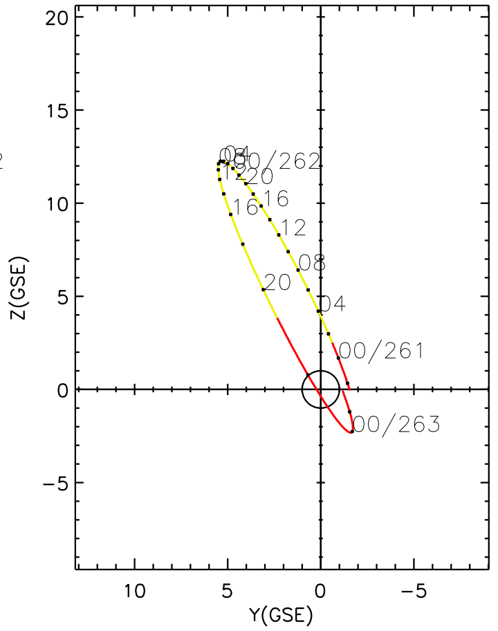
CLUSTER 2 orbit 2023 260 (09/17) 21:26 UT to 2023 263 (09/20) 03:41 UT
