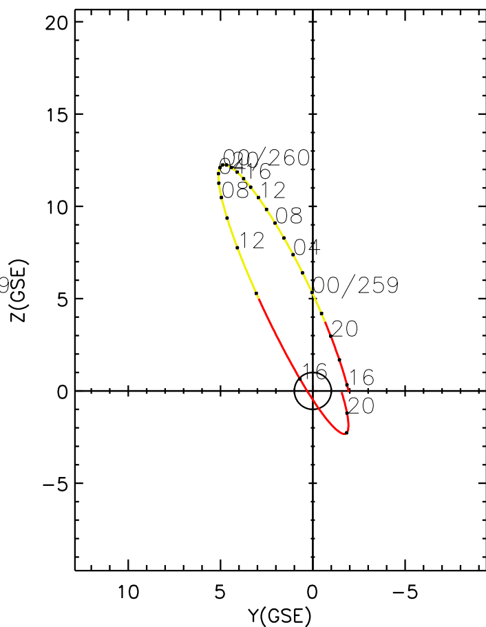
CLUSTER 2 orbit 2023 258 (09/15) 15:26 UT to 2023 260 (09/17) 21:41 UT
