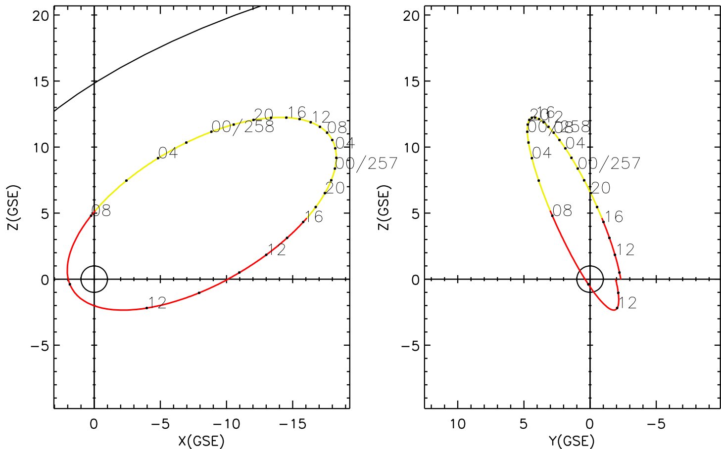
CLUSTER 2 orbit 2023 256 (09/13) 09:16 UT to 2023 258 (09/15) 15:31 UT
