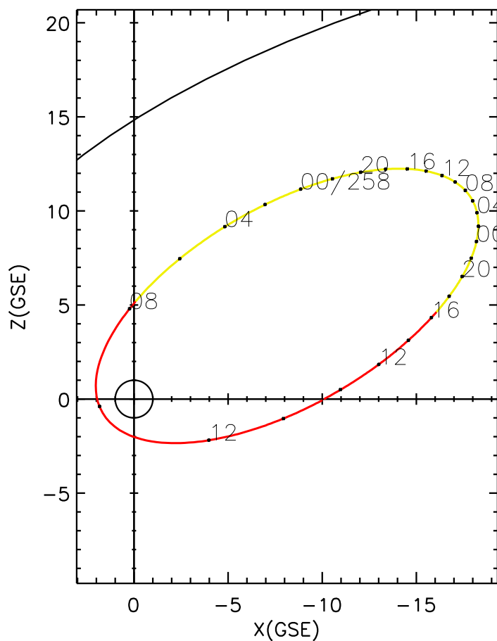
CLUSTER 2 orbit 2023 256 (09/13) 09:16 UT to 2023 258 (09/15) 15:26 UT
