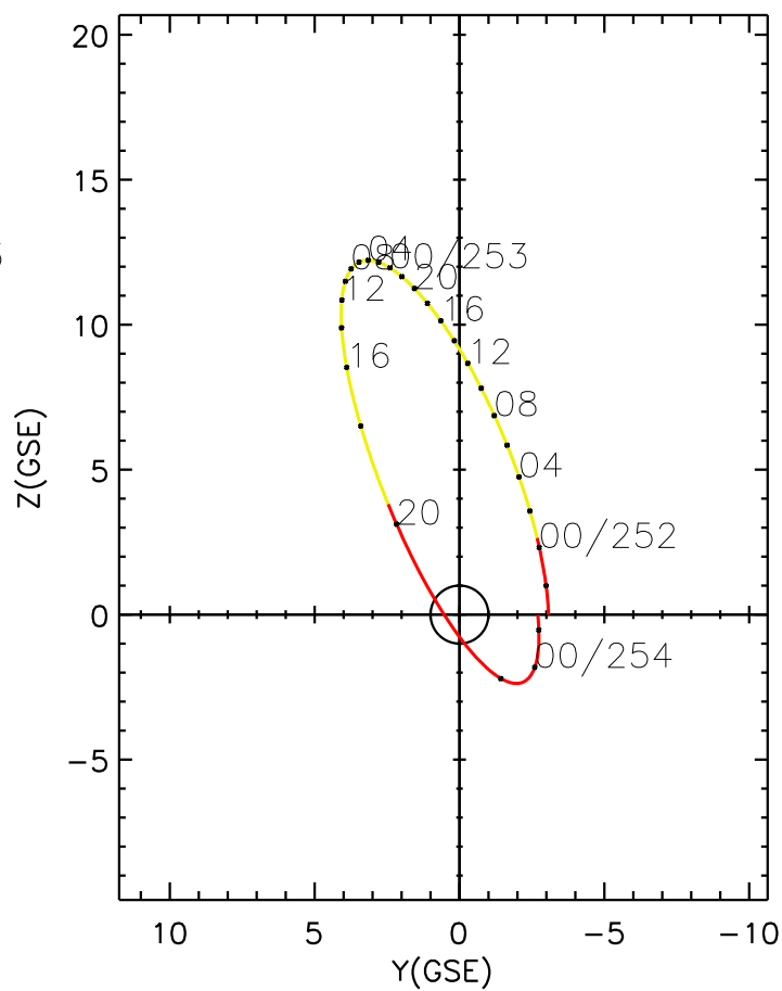
CLUSTER 2 orbit 2023 251 (09/08) 20:31 UT to 2023 254 (09/11) 02:46 UT
