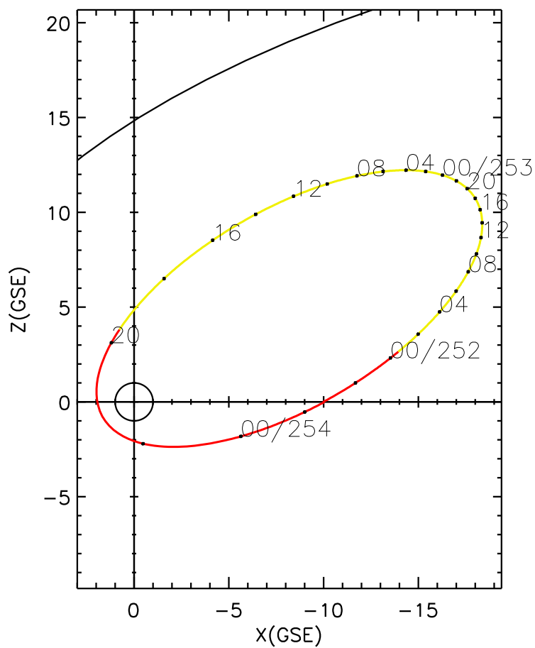
CLUSTER 2 orbit 2023 251 (09/08) 20:31 UT to 2023 254 (09/11) 02:46 UT
