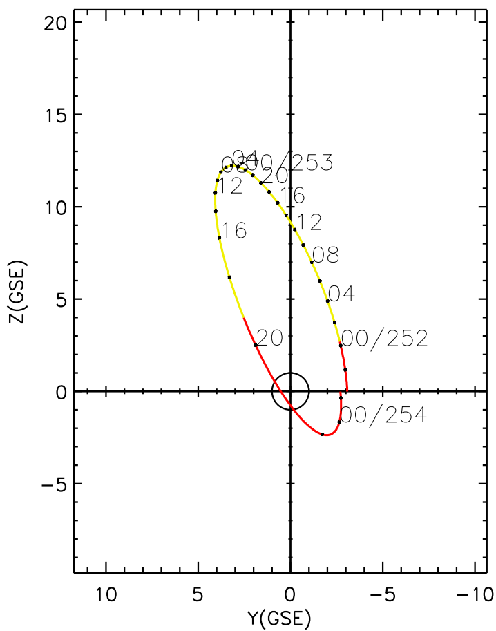
CLUSTER 2 orbit 2023 251 (09/08) 20:16 UT to 2023 254 (09/11) 02:31 UT
