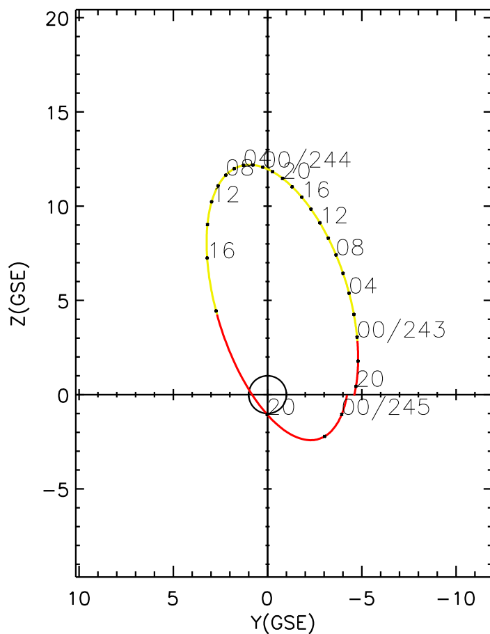
CLUSTER 2 orbit 2023 242 (08/30) 19:16 UT to 2023 245 (09/02) 01:31 UT
