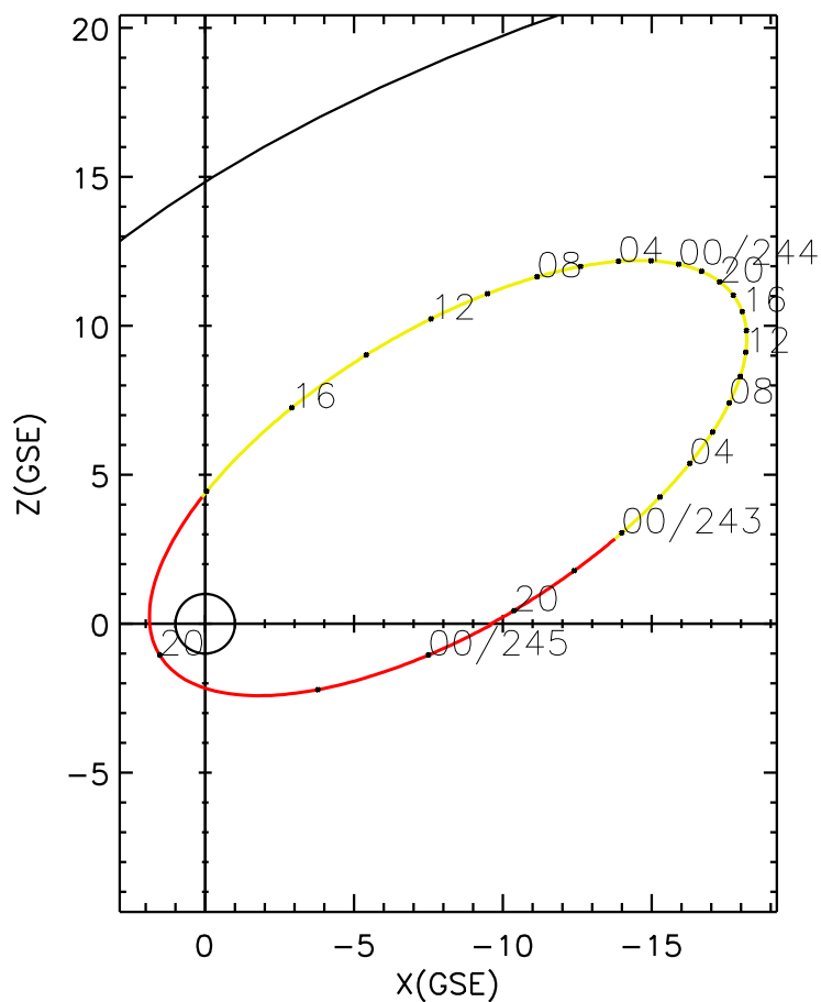
CLUSTER 2 orbit 2023 242 (08/30) 19:16 UT to 2023 245 (09/02) 01:31 UT
