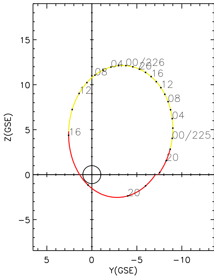
CLUSTER 2 orbit 2023 224 (08/12) 17:36 UT to 2023 226 (08/14) 23:51 UT
