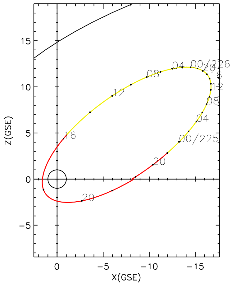
CLUSTER 2 orbit 2023 224 (08/12) 17:36 UT to 2023 226 (08/14) 23:51 UT
