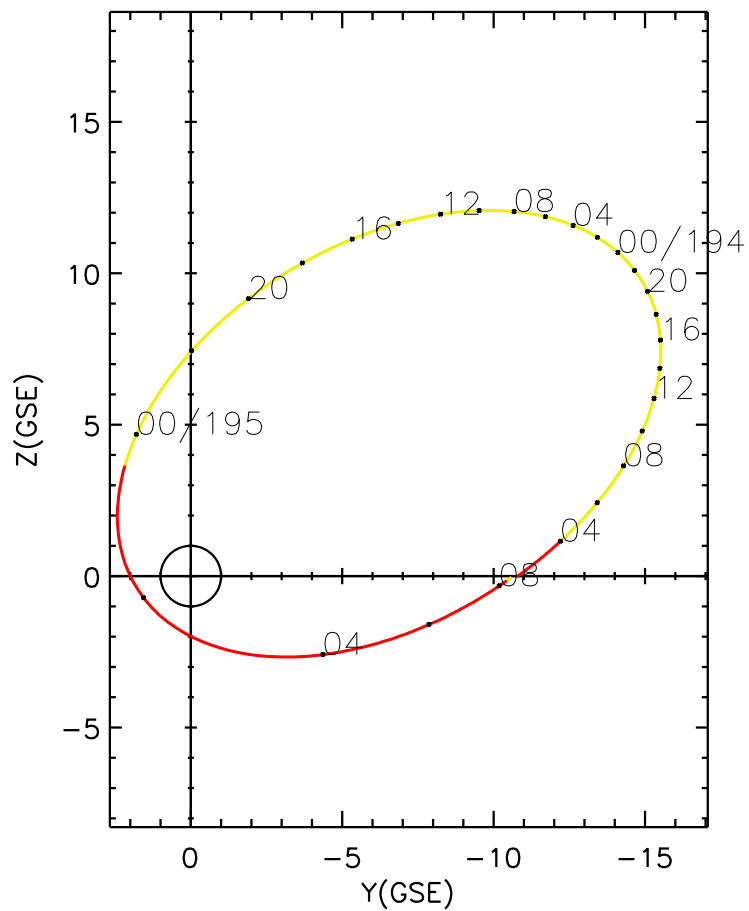
CLUSTER 2 orbit 2023 193 (07/12) 02:11 UT to 2023 195 (07/14) 08:26 UT
