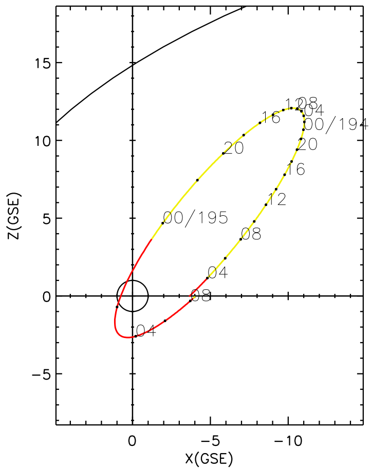
CLUSTER 2 orbit 2023 193 (07/12) 02:11 UT to 2023 195 (07/14) 08:26 UT
