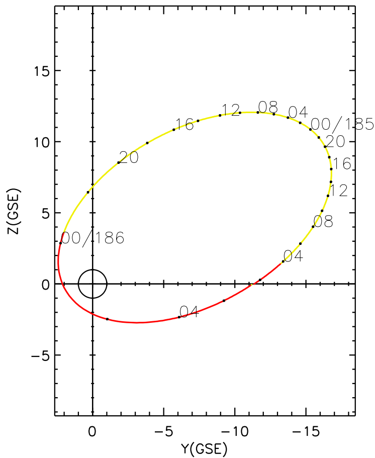
CLUSTER 2 orbit 2023 184 (07/03) 01:31 UT to 2023 186 (07/05) 07:46 UT
