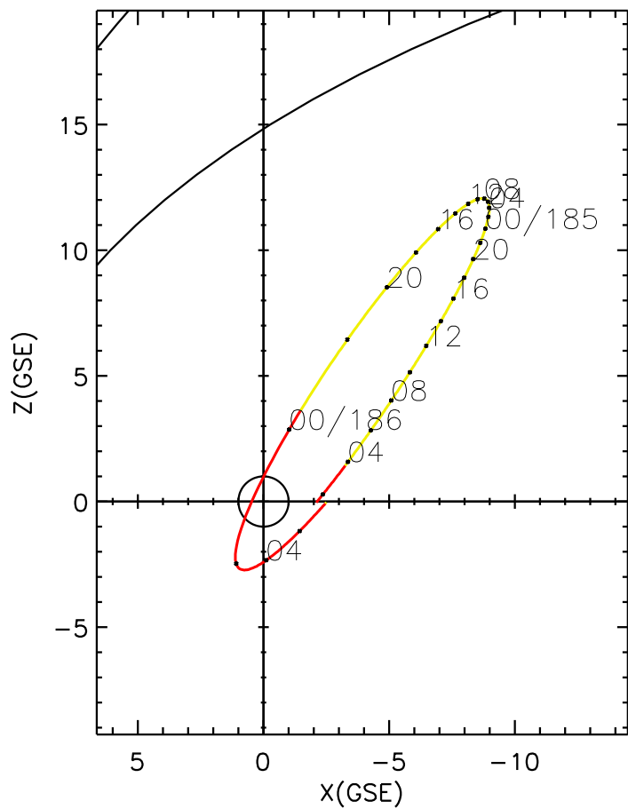
CLUSTER 2 orbit 2023 184 (07/03) 01:31 UT to 2023 186 (07/05) 07:46 UT
