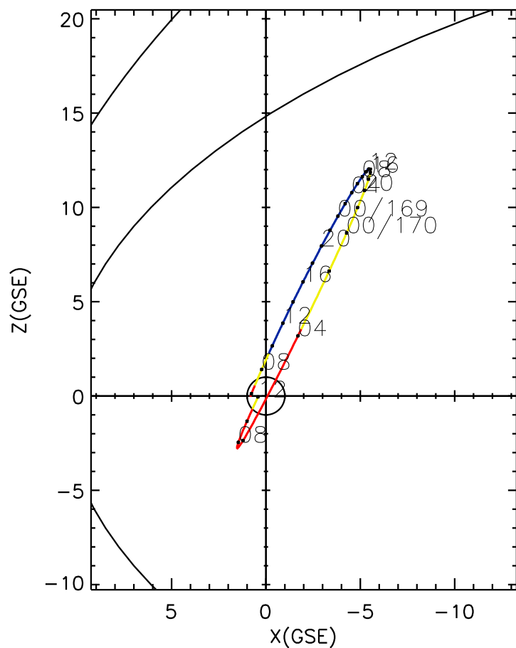
CLUSTER 2 orbit 2023 168 (06/17) 05:46 UT to 2023 170 (06/19) 12:01 UT
