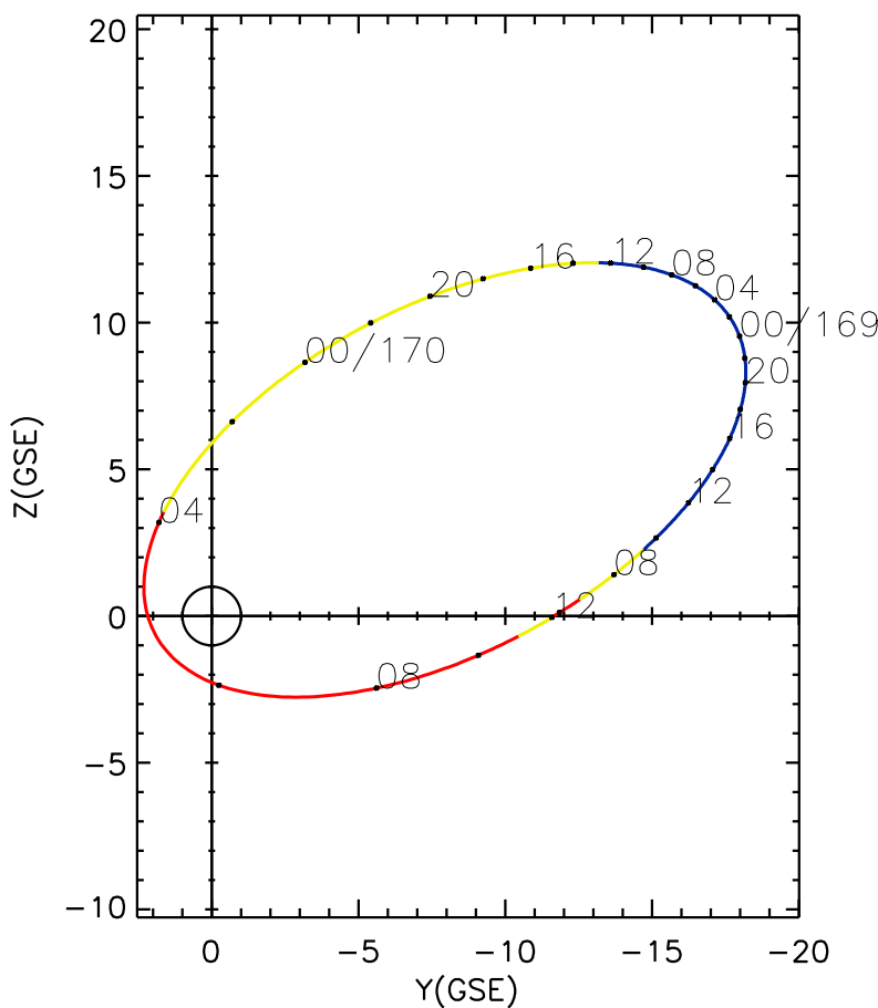
CLUSTER 2 orbit 2023 168 (06/17) 05:46 UT to 2023 170 (06/19) 12:01 UT
