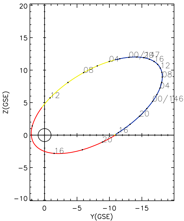
CLUSTER 2 orbit 2023 145 (05/25) 15:21 UT to 2023 147 (05/27) 21:36 UT
