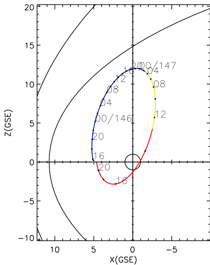
CLUSTER 2 orbit 2023 145 (05/25) 15:21 UT to 2023 147 (05/27) 21:36 UT
