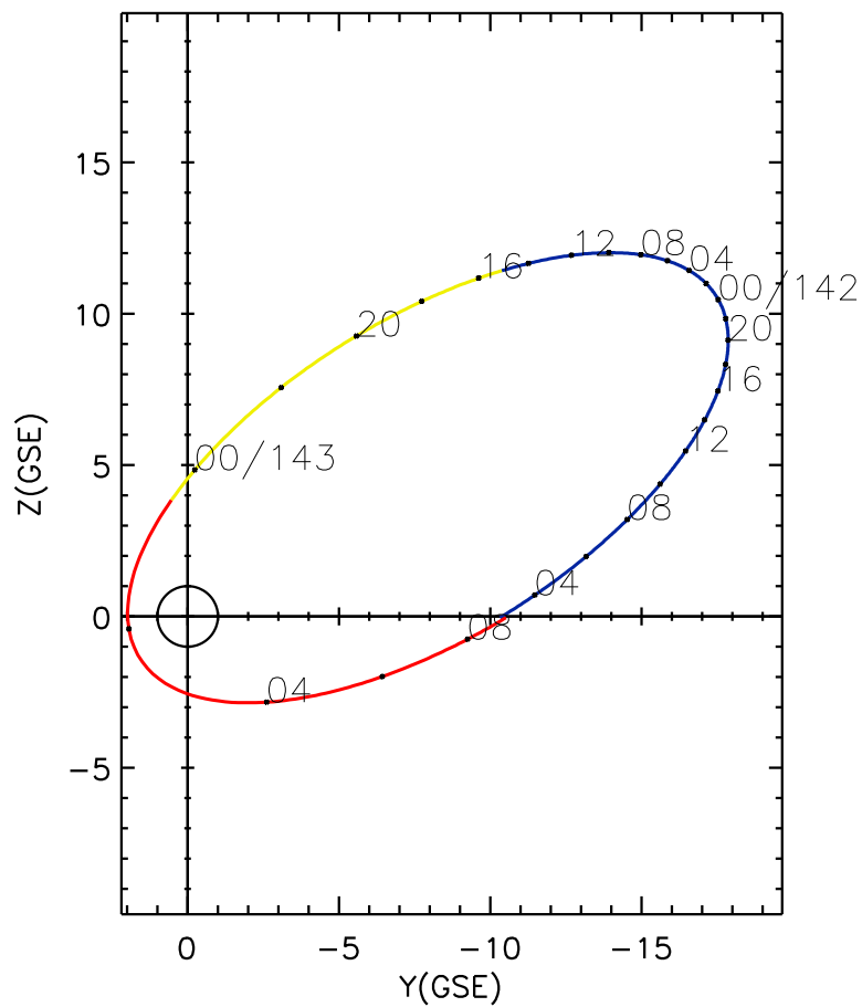
CLUSTER 2 orbit 2023 141 (05/21) 02:51 UT to 2023 143 (05/23) 09:06 UT
