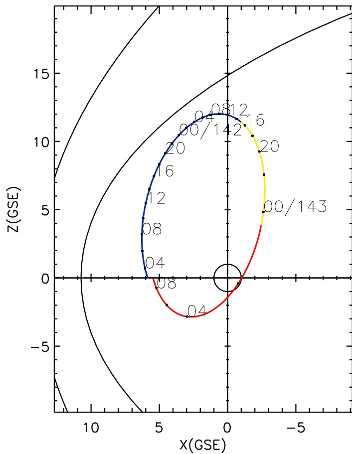
CLUSTER 2 orbit 2023 141 (05/21) 02:51 UT to 2023 143 (05/23) 09:06 UT
