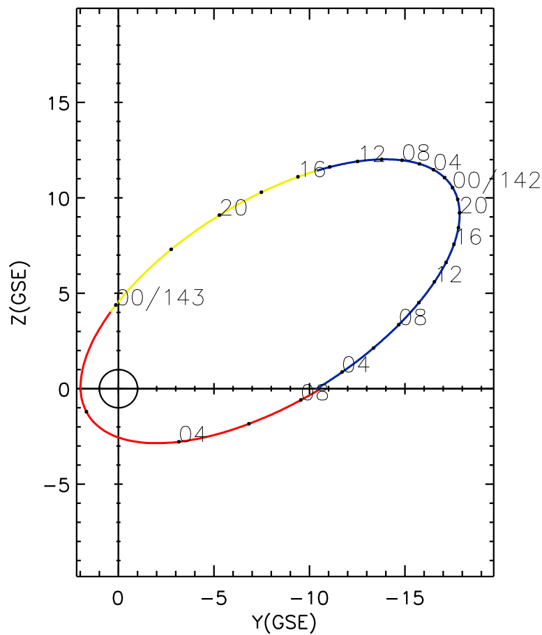
CLUSTER 2 orbit 2023 141 (05/21) 02:36 UT to 2023 143 (05/23) 08:51 UT
