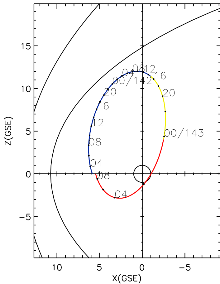
CLUSTER 2 orbit 2023 141 (05/21) 02:36 UT to 2023 143 (05/23) 08:51 UT
