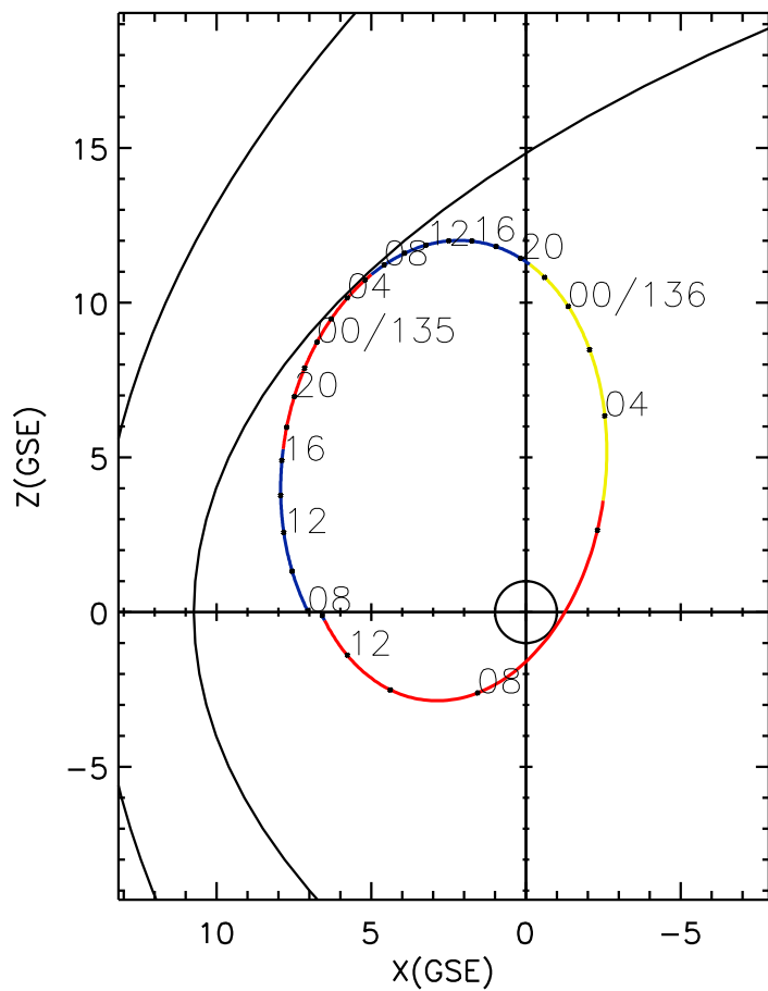
CLUSTER 2 orbit 2023 134 (05/14) 07:56 UT to 2023 136 (05/16) 14:06 UT
