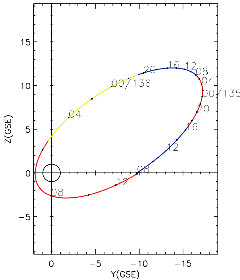
CLUSTER 2 orbit 2023 134 (05/14) 07:56 UT to 2023 136 (05/16) 14:06 UT
