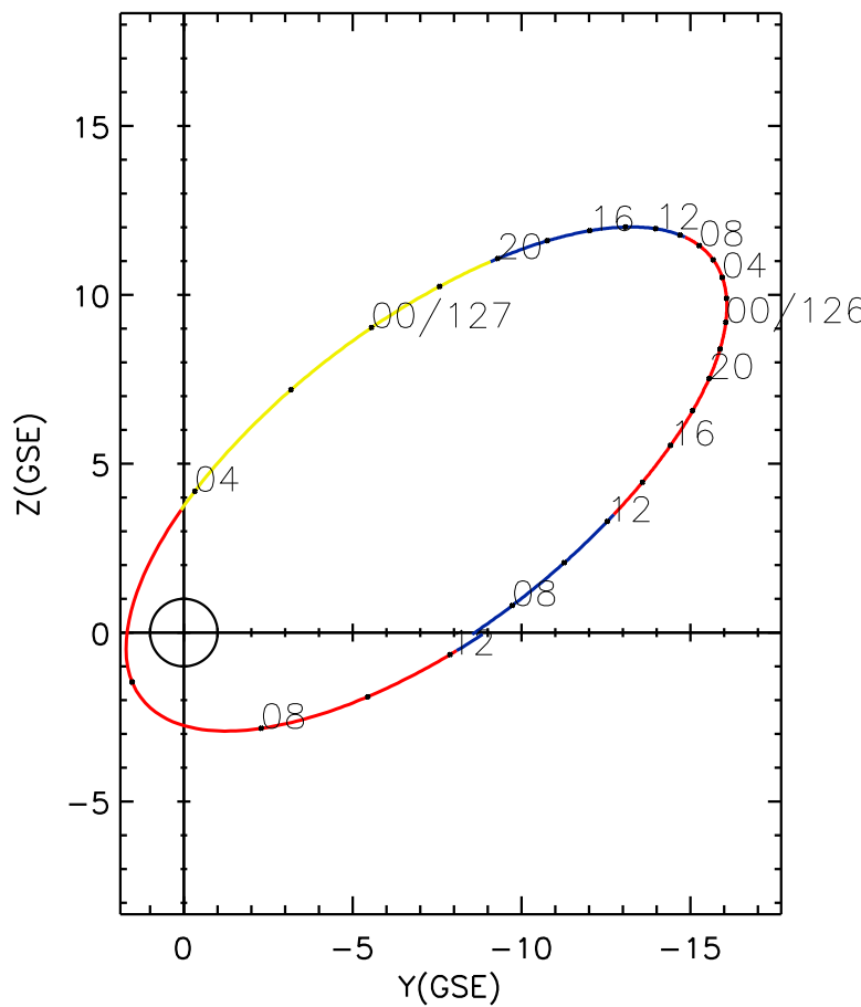
CLUSTER 2 orbit 2023 125 (05/05) 06:41 UT to 2023 127 (05/07) 12:56 UT
