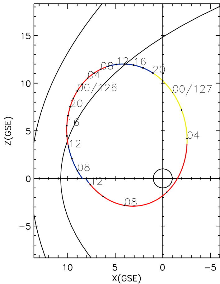
CLUSTER 2 orbit 2023 125 (05/05) 06:41 UT to 2023 127 (05/07) 12:56 UT
