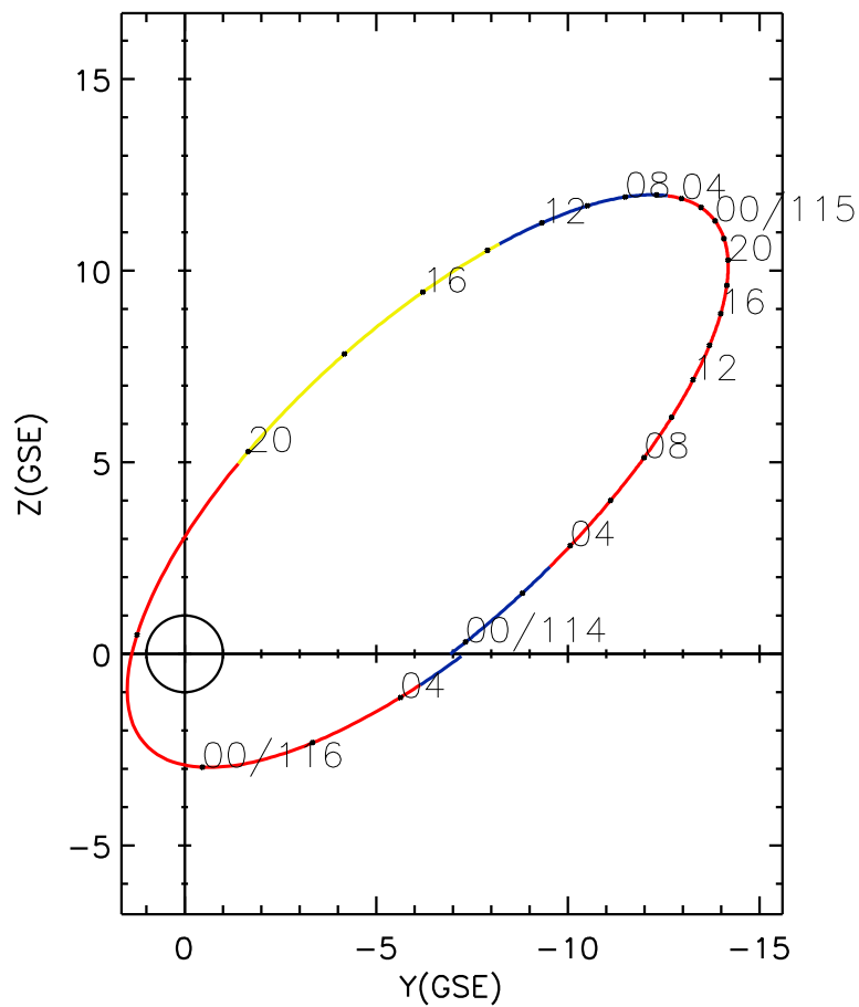
CLUSTER 2 orbit 2023 113 (04/23) 23:31 UT to 2023 116 (04/26) 05:41 UT
