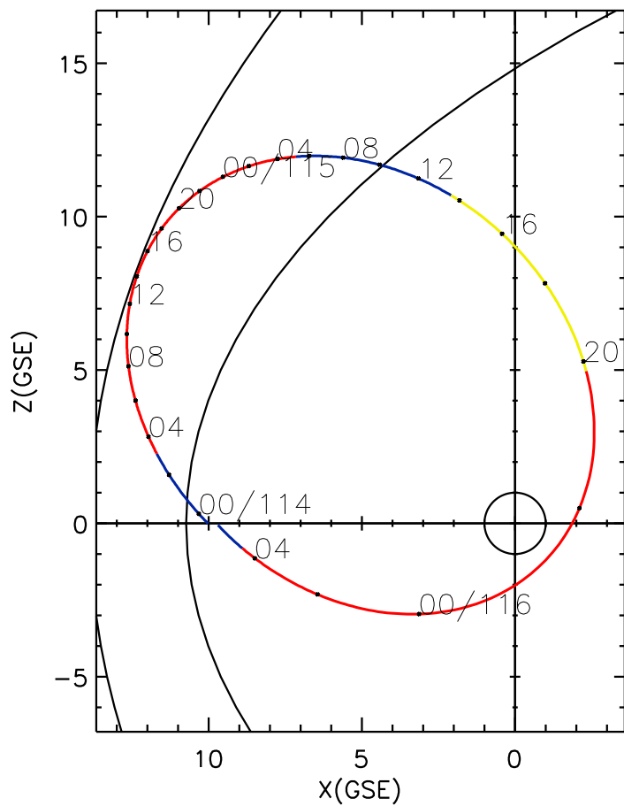
CLUSTER 2 orbit 2023 113 (04/23) 23:31 UT to 2023 116 (04/26) 05:41 UT
