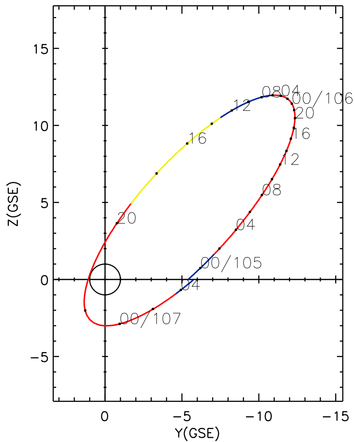
CLUSTER 2 orbit 2023 104 (04/14) 22:46 UT to 2023 107 (04/17) 05:01 UT
