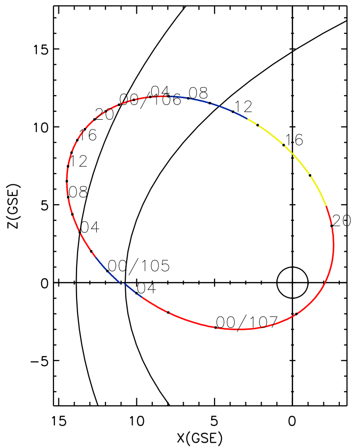
CLUSTER 2 orbit 2023 104 (04/14) 22:46 UT to 2023 107 (04/17) 05:01 UT
