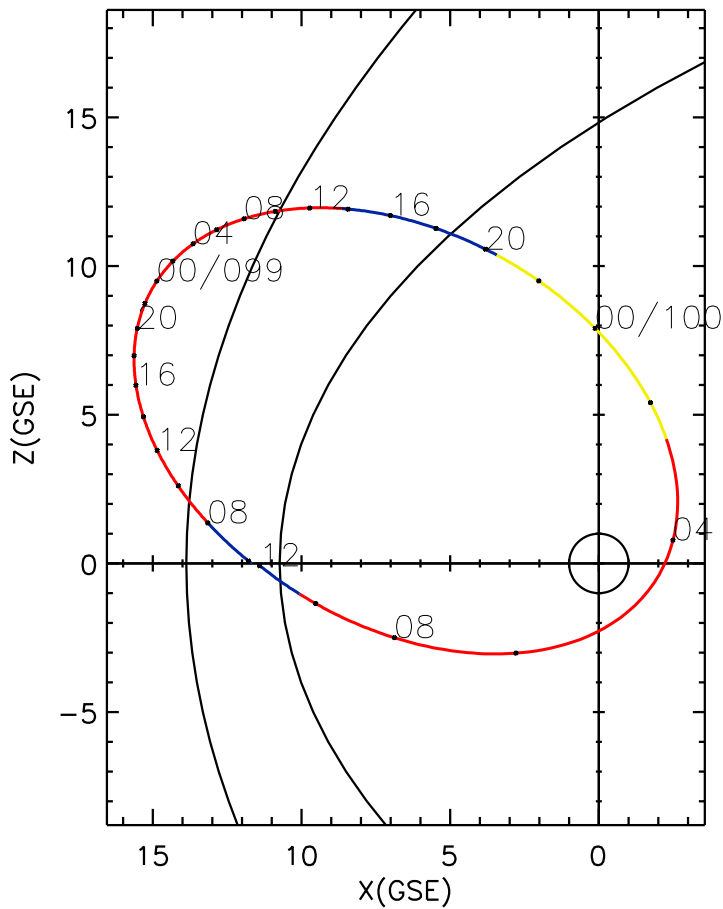
CLUSTER 2 orbit 2023 098 (04/08) 05:51 UT to 2023 100 (04/10) 12:06 UT
