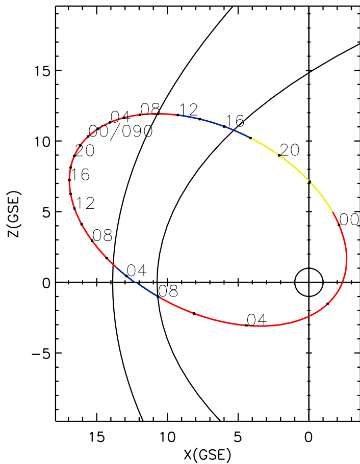
CLUSTER 2 orbit 2023 089 (03/30) 03:16 UT to 2023 091 (04/01) 09:31 UT
