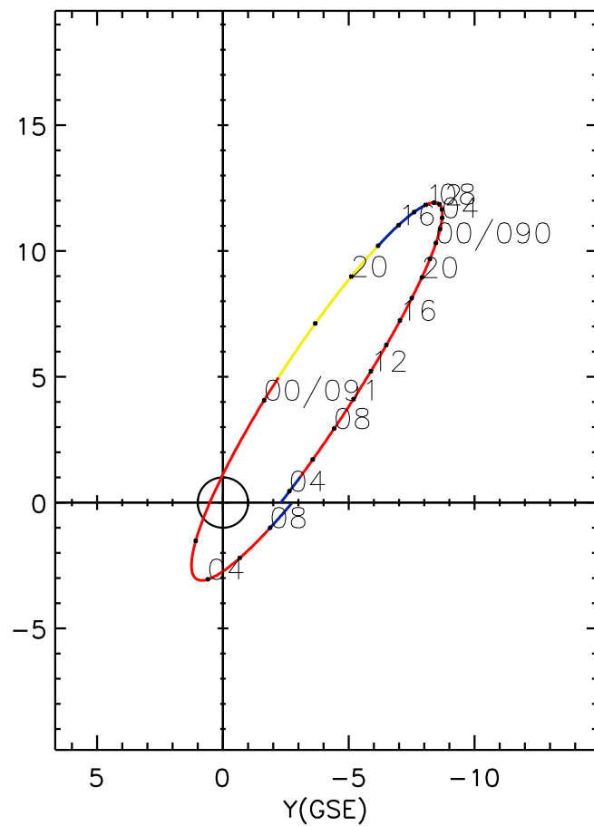
CLUSTER 2 orbit 2023 089 (03/30) 03:16 UT to 2023 091 (04/01) 09:31 UT
