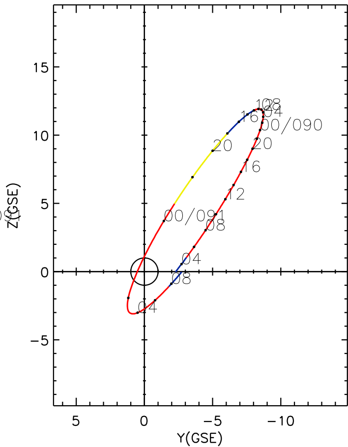
CLUSTER 2 orbit 2023 089 (03/30) 03:06 UT to 2023 091 (04/01) 09:21 UT
