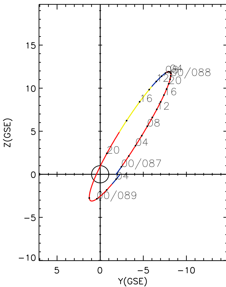
CLUSTER 2 orbit 2023 086 (03/27) 22:36 UT to 2023 089 (03/30) 04:51 UT
