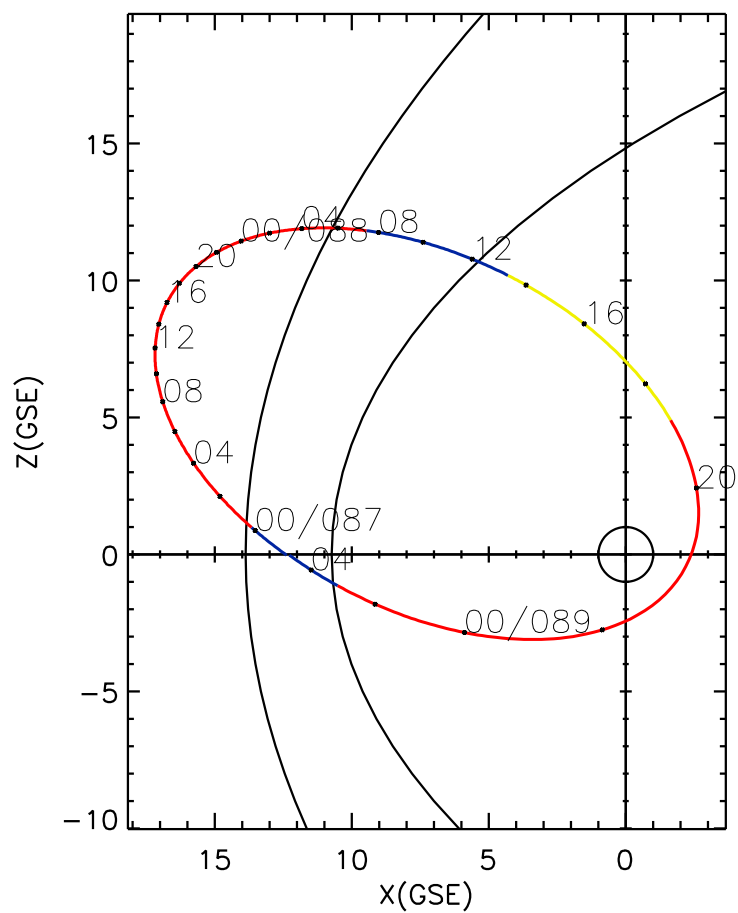
CLUSTER 2 orbit 2023 086 (03/27) 22:36 UT to 2023 089 (03/30) 04:51 UT
