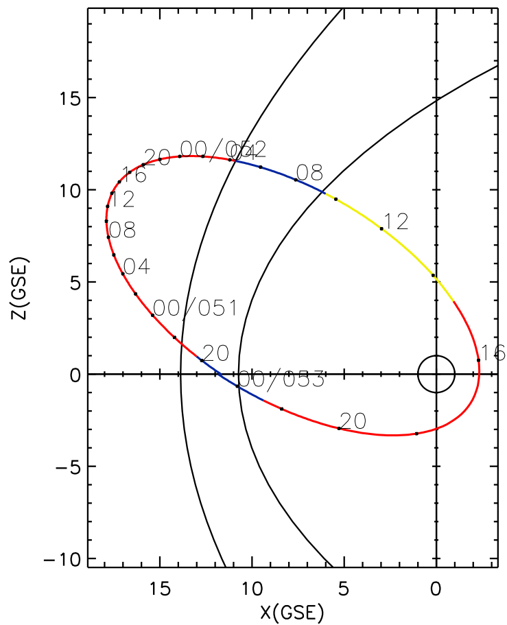
CLUSTER 2 orbit 2023 050 (02/19) 18:46 UT to 2023 053 (02/22) 01:01 UT
