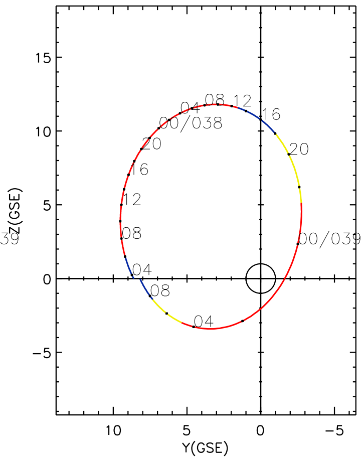
CLUSTER 2 orbit 2023 037 (02/06) 03:36 UT to 2023 039 (02/08) 09:51 UT
