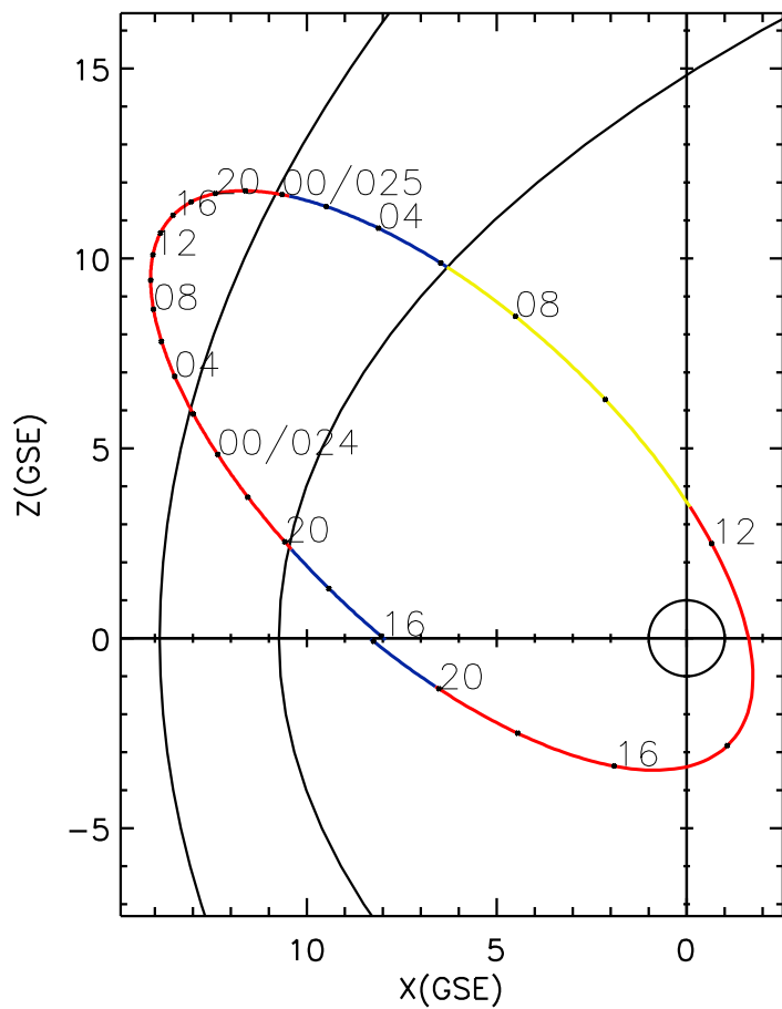
CLUSTER 2 orbit 2023 023 (01/23) 15:51 UT to 2023 025 (01/25) 22:06 UT
