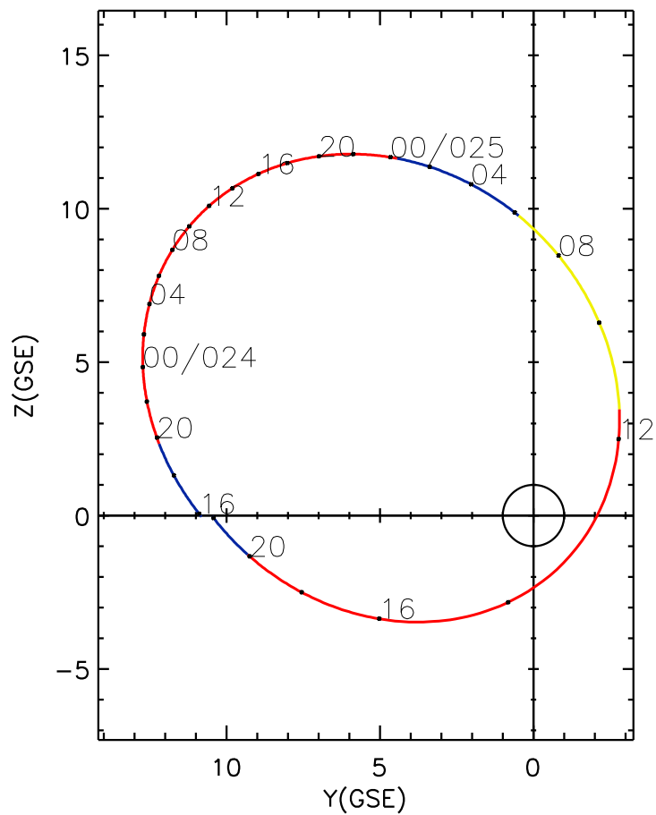
CLUSTER 2 orbit 2023 023 (01/23) 15:51 UT to 2023 025 (01/25) 22:06 UT
