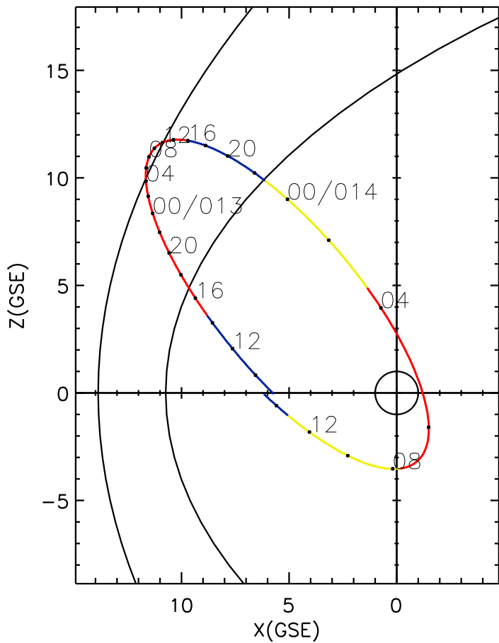
CLUSTER 2 orbit 2023 012 (01/12) 08:36 UT to 2023 014 (01/14) 14:51 UT
