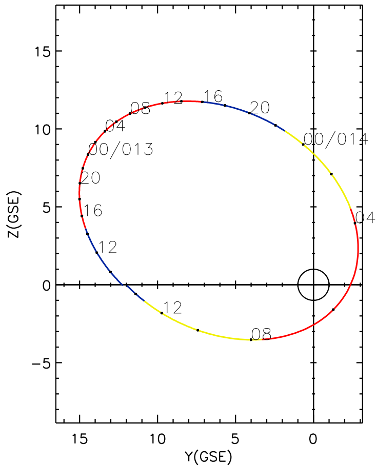
CLUSTER 2 orbit 2023 012 (01/12) 08:36 UT to 2023 014 (01/14) 14:51 UT
