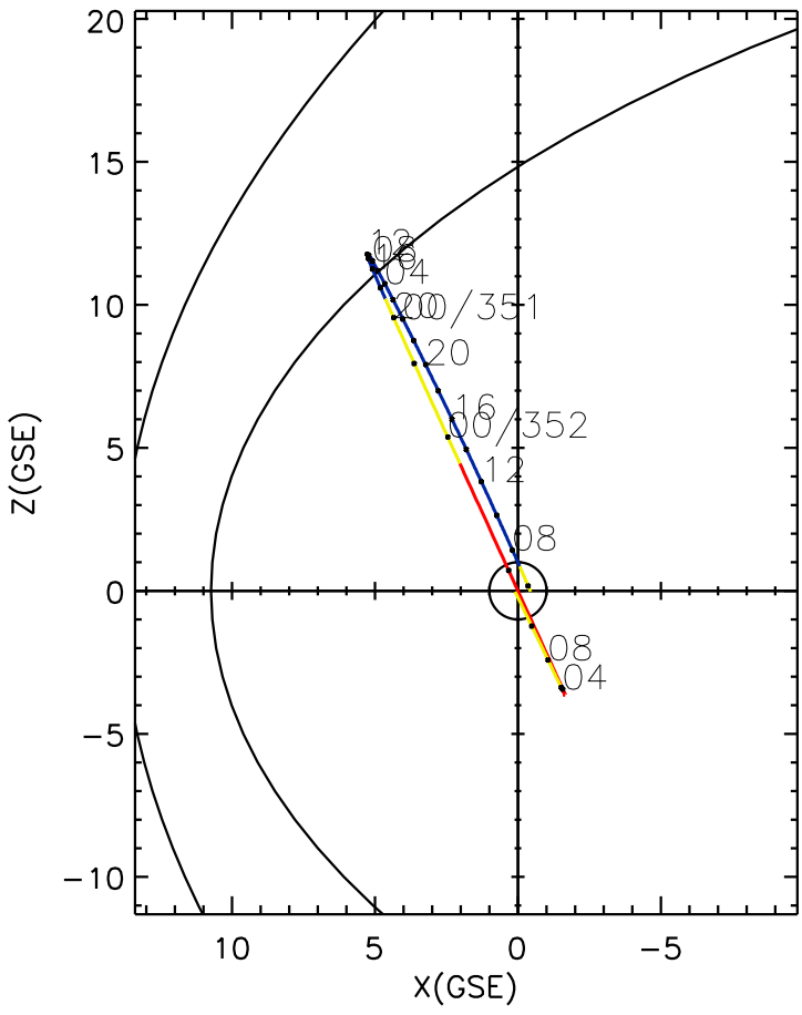
CLUSTER 2 orbit 2022 350 (12/16) 05:41 UT to 2022 352 (12/18) 11:56 UT
