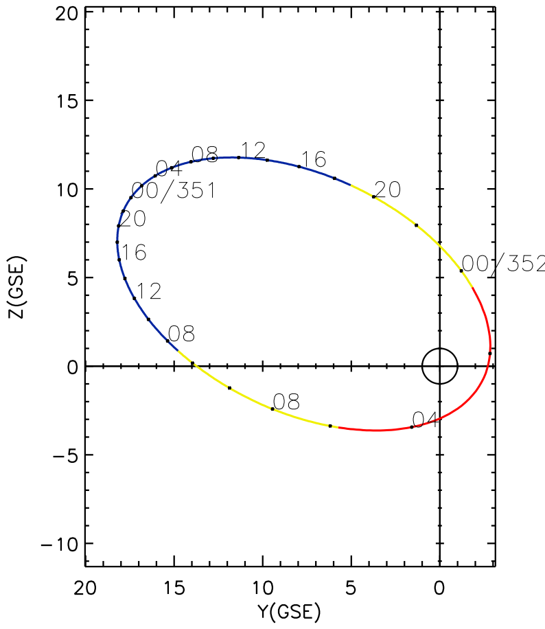
CLUSTER 2 orbit 2022 350 (12/16) 05:41 UT to 2022 352 (12/18) 11:56 UT
