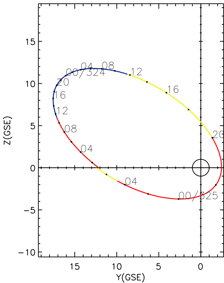
CLUSTER 2 orbit 2022 323 (11/19) 01:01 UT to 2022 325 (11/21) 07:11 UT
