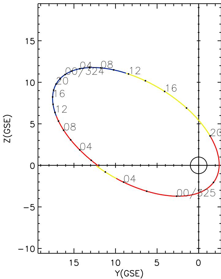
CLUSTER 2 orbit 2022 323 (11/19) 00:56 UT to 2022 325 (11/21) 07:11 UT
