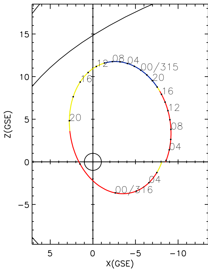
CLUSTER 2 orbit 2022 314 (11/10) 01:41 UT to 2022 316 (11/12) 07:56 UT
