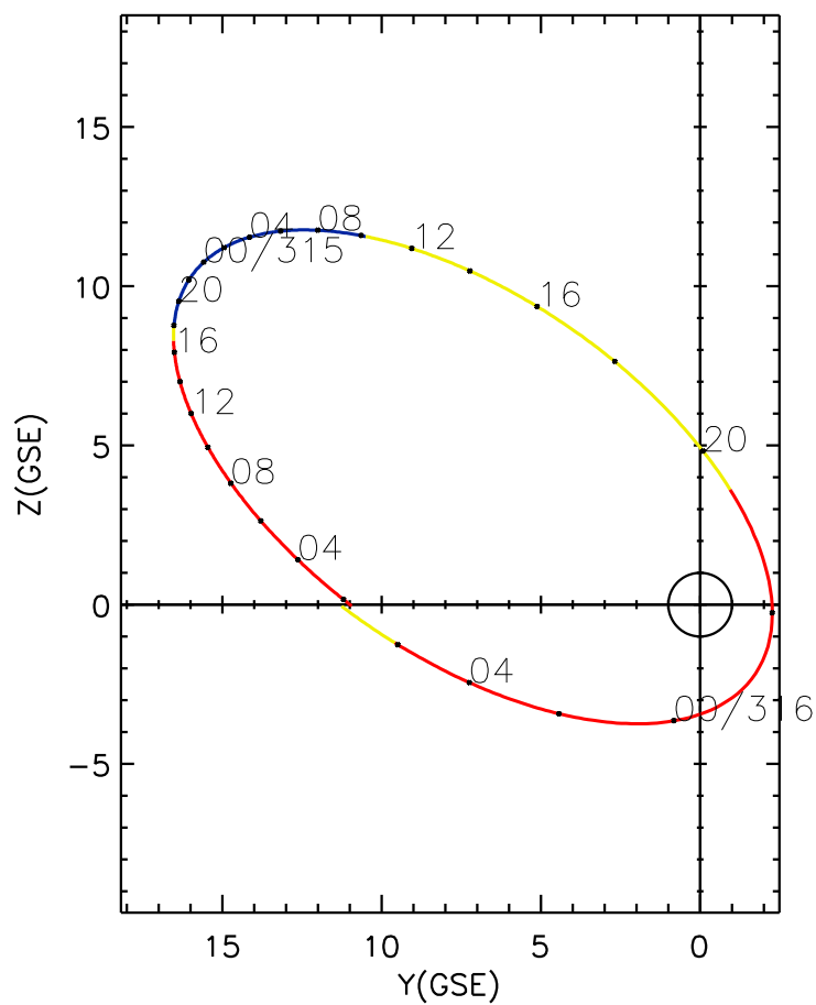
CLUSTER 2 orbit 2022 314 (11/10) 01:41 UT to 2022 316 (11/12) 07:56 UT
