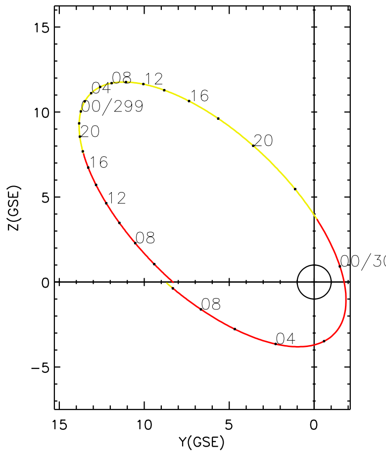
CLUSTER 2 orbit 2022 298 (10/25) 04:16 UT to 2022 300 (10/27) 10:31 UT
