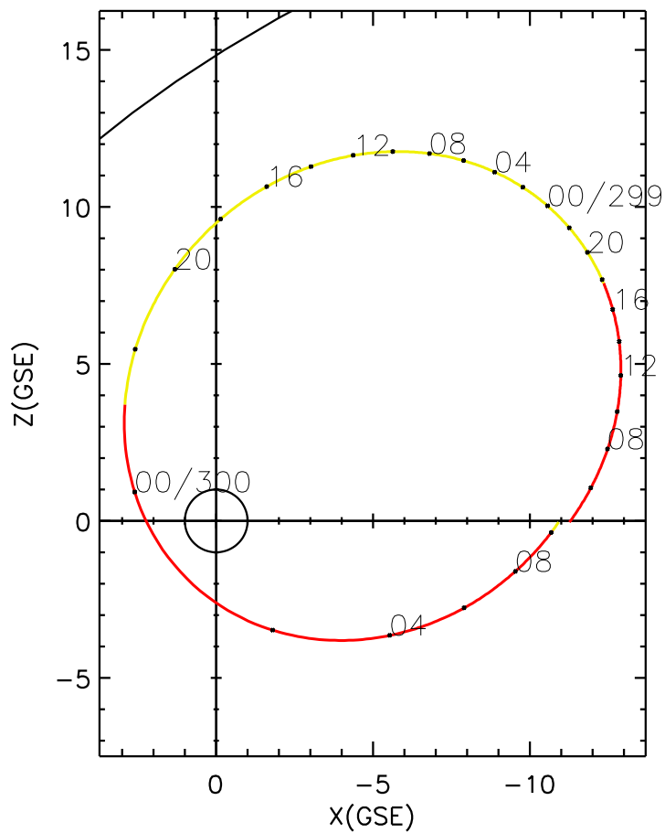
CLUSTER 2 orbit 2022 298 (10/25) 04:16 UT to 2022 300 (10/27) 10:31 UT
