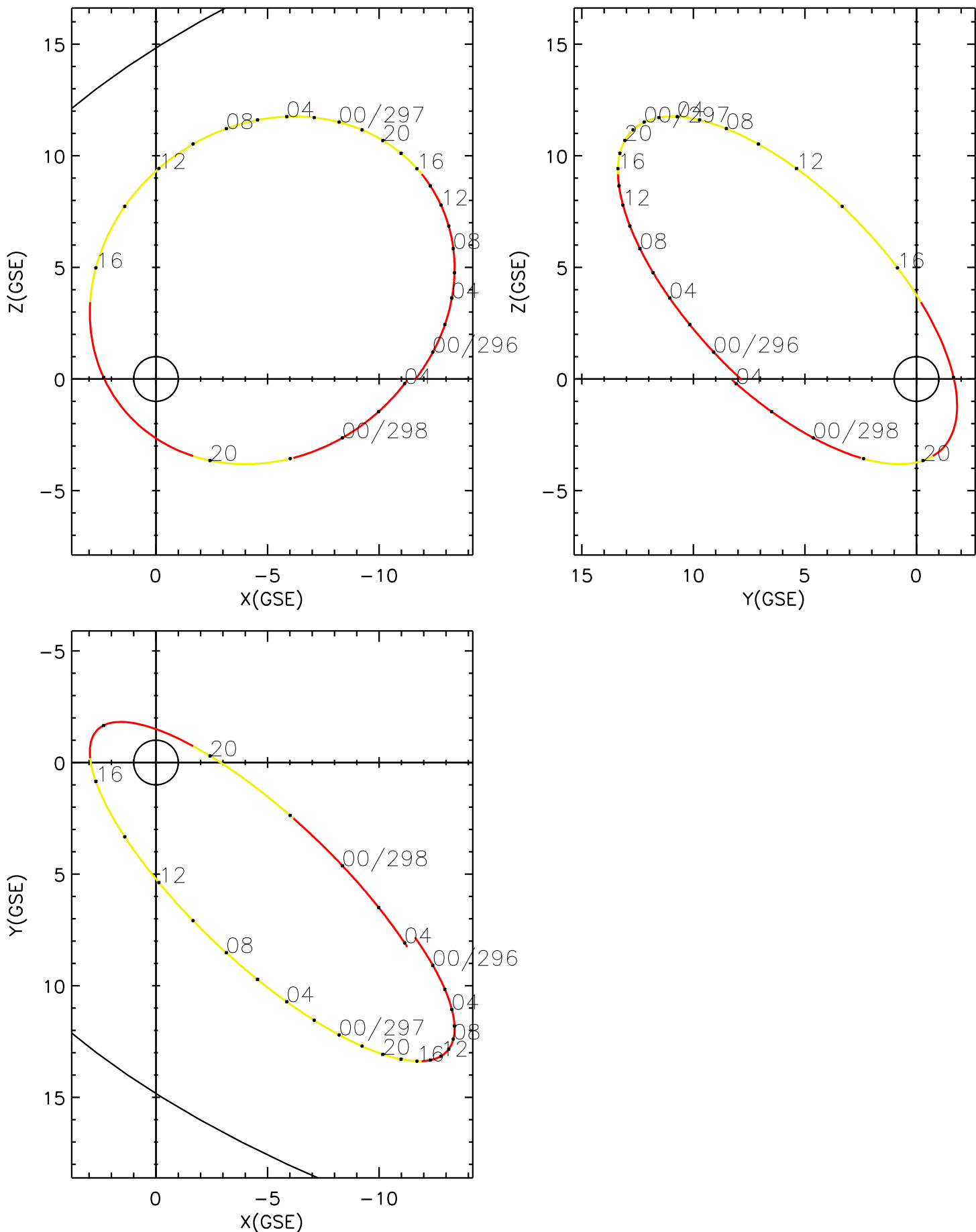
CLUSTER 2 orbit 2022 295 (10/22) 22:01 UT to 2022 298 (10/25) 04:16 UT
