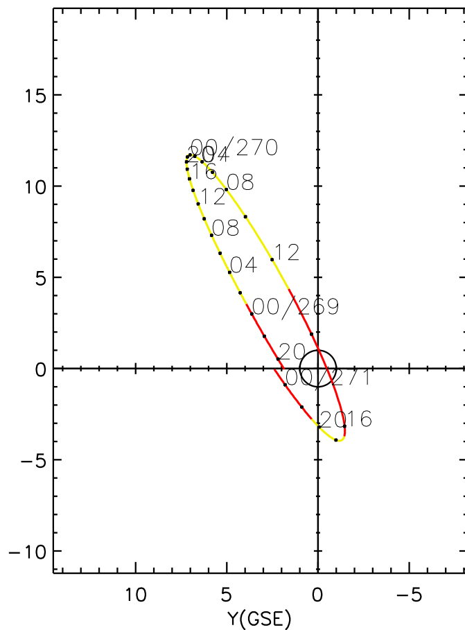
CLUSTER 2 orbit 2022 268 (09/25) 19:06 UT to 2022 271 (09/28) 01:21 UT
