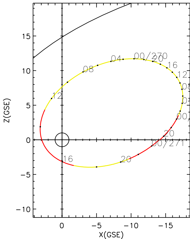
CLUSTER 2 orbit 2022 268 (09/25) 19:06 UT to 2022 271 (09/28) 01:21 UT
