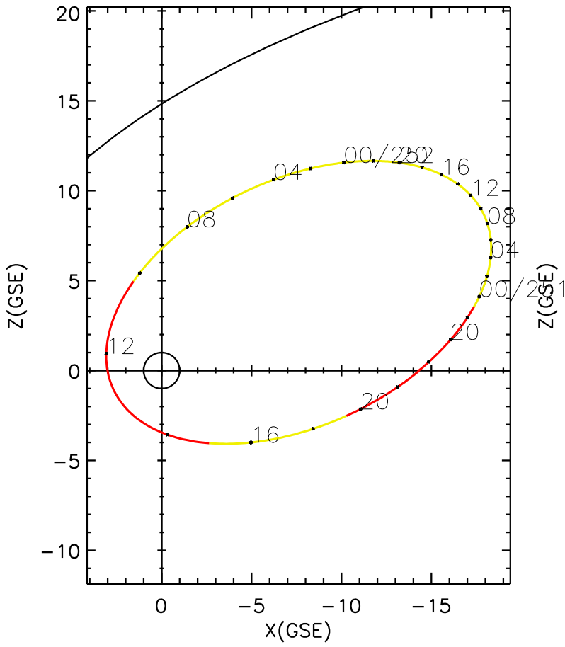
CLUSTER 2 orbit 2022 250 (09/07) 17:11 UT to 2022 252 (09/09) 23:26 UT
