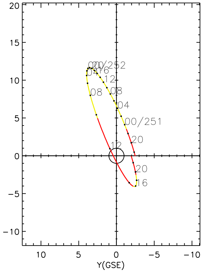
CLUSTER 2 orbit 2022 250 (09/07) 17:11 UT to 2022 252 (09/09) 23:26 UT
