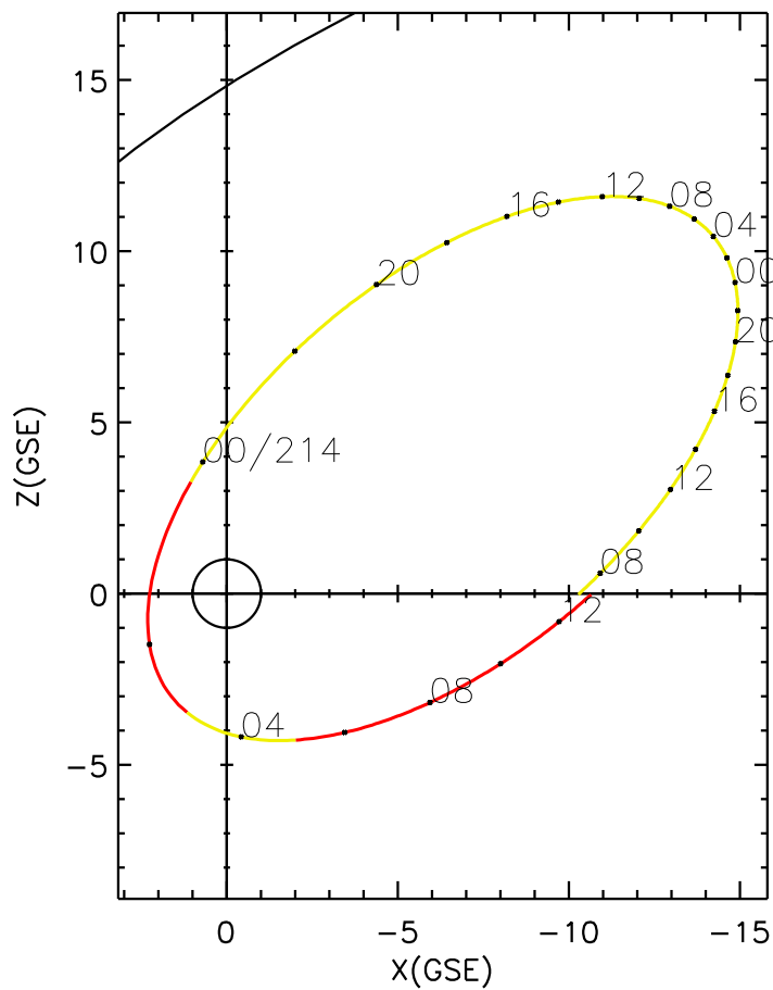
CLUSTER 2 orbit 2022 212 (07/31) 07:01 UT to 2022 214 (08/02) 13:16 UT
