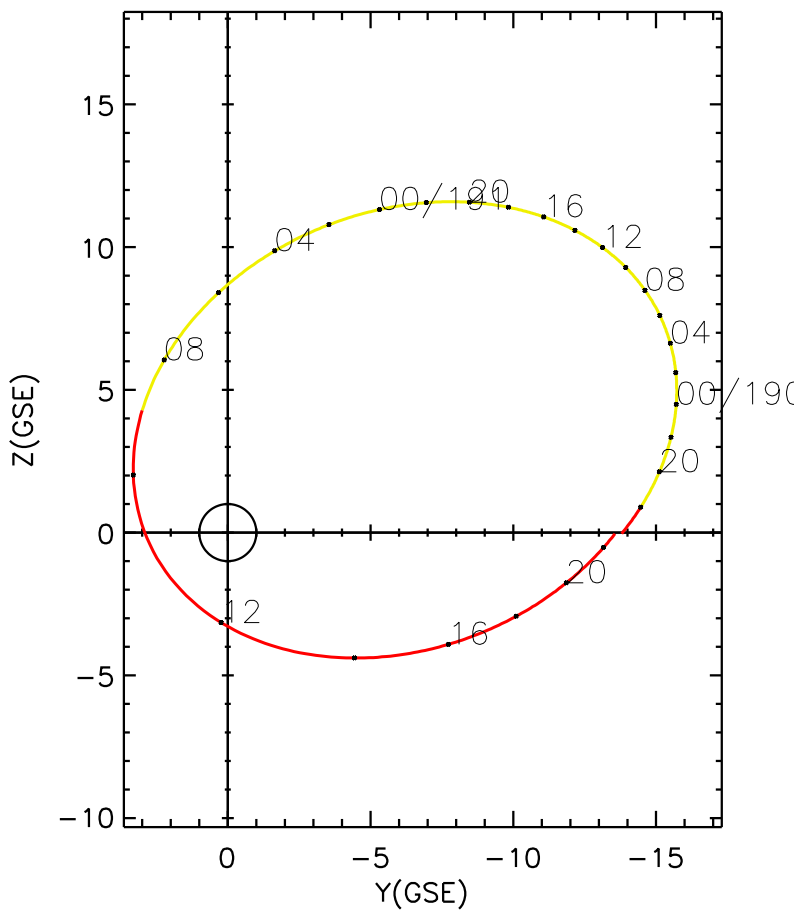
CLUSTER 2 orbit 2022 189 (07/08) 16:31 UT to 2022 191 (07/10) 22:46 UT
