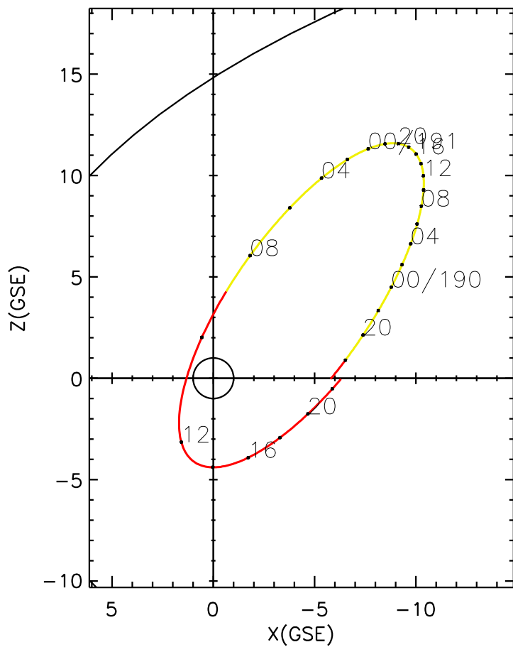
CLUSTER 2 orbit 2022 189 (07/08) 16:31 UT to 2022 191 (07/10) 22:46 UT
