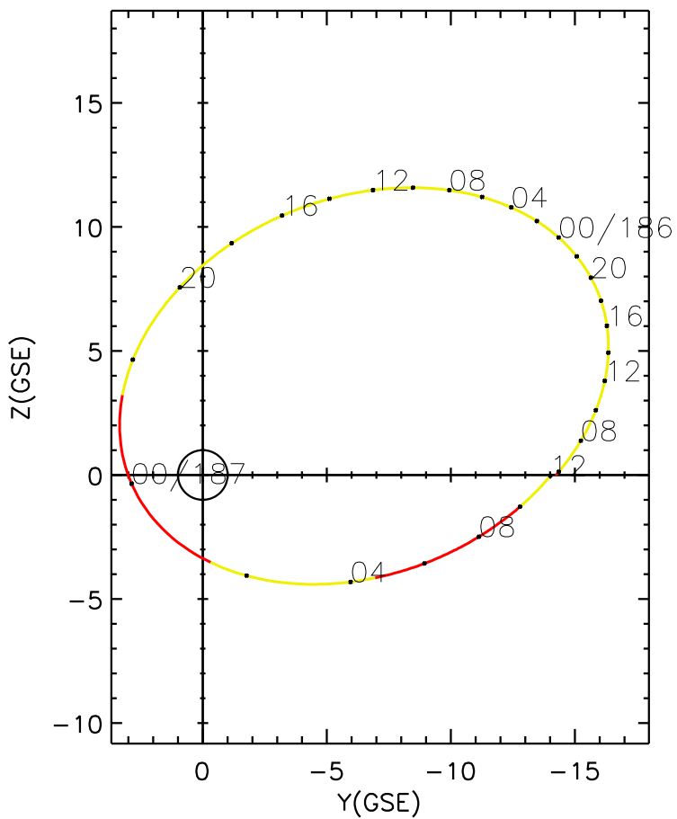
CLUSTER 2 orbit 2022 185 (07/04) 05:46 UT to 2022 187 (07/06) 12:01 UT
