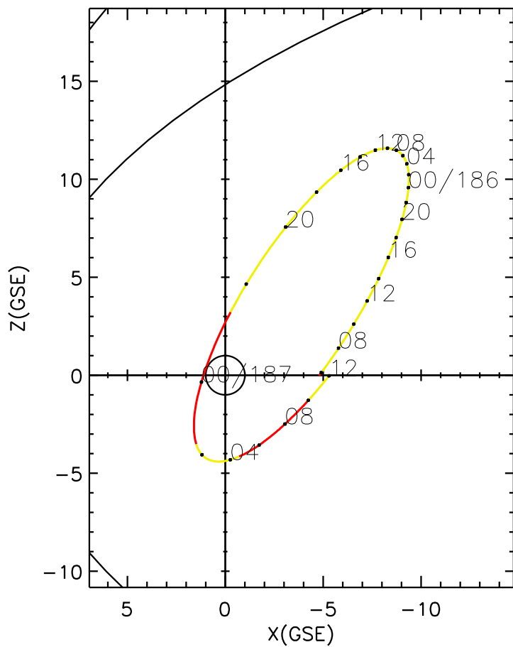
CLUSTER 2 orbit 2022 185 (07/04) 05:46 UT to 2022 187 (07/06) 12:01 UT
