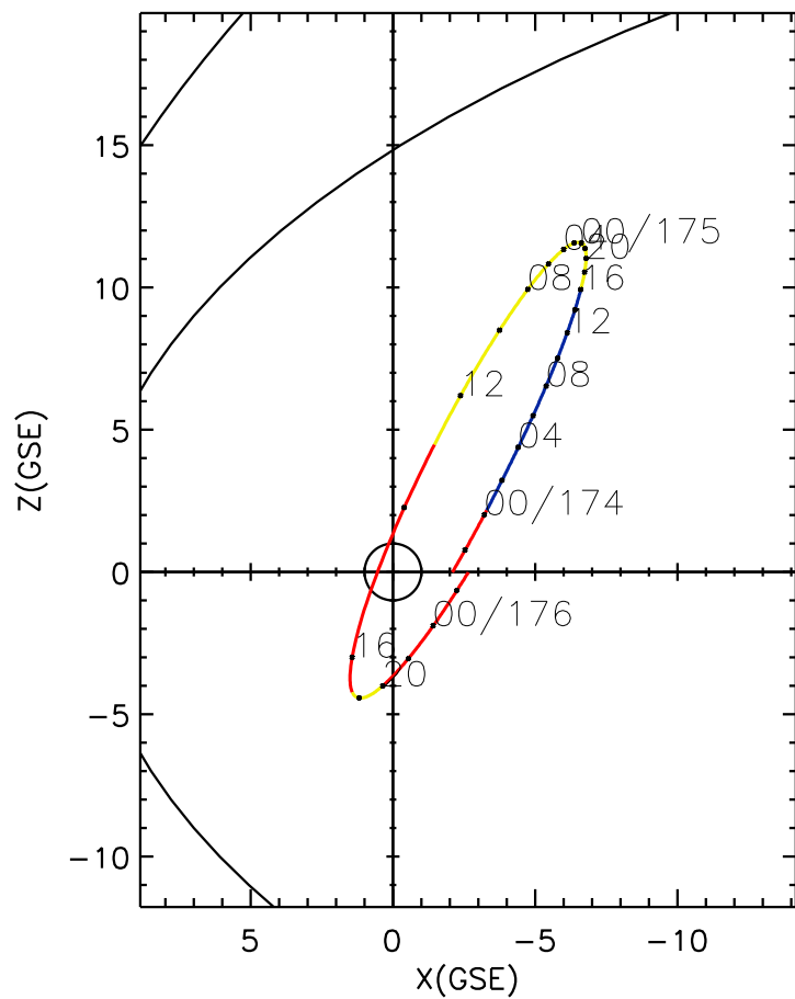
CLUSTER 2 orbit 2022 173 (06/22) 20:46 UT to 2022 176 (06/25) 03:01 UT
