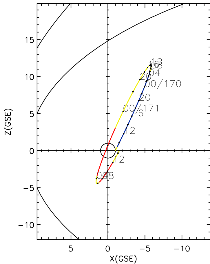
CLUSTER 2 orbit 2022 169 (06/18) 08:16 UT to 2022 171 (06/20) 14:31 UT
