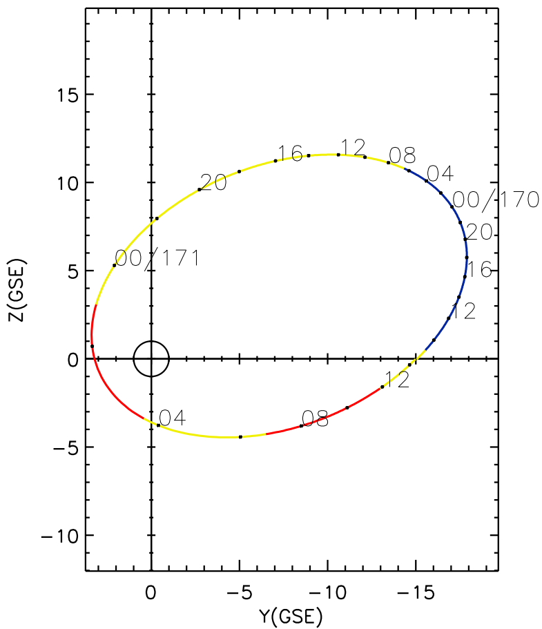
CLUSTER 2 orbit 2022 169 (06/18) 08:16 UT to 2022 171 (06/20) 14:31 UT
