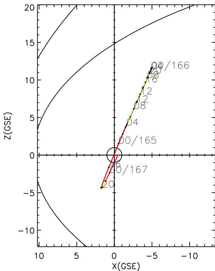
CLUSTER 2 orbit 2022 164 (06/13) 21:31 UT to 2022 167 (06/16) 03:46 UT
