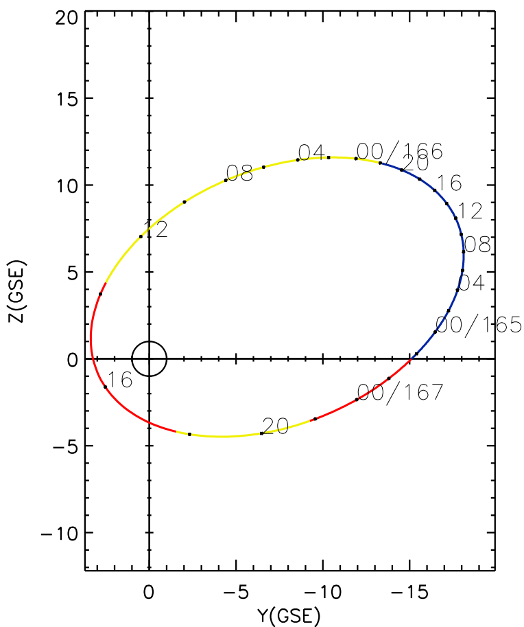
CLUSTER 2 orbit 2022 164 (06/13) 21:31 UT to 2022 167 (06/16) 03:46 UT
