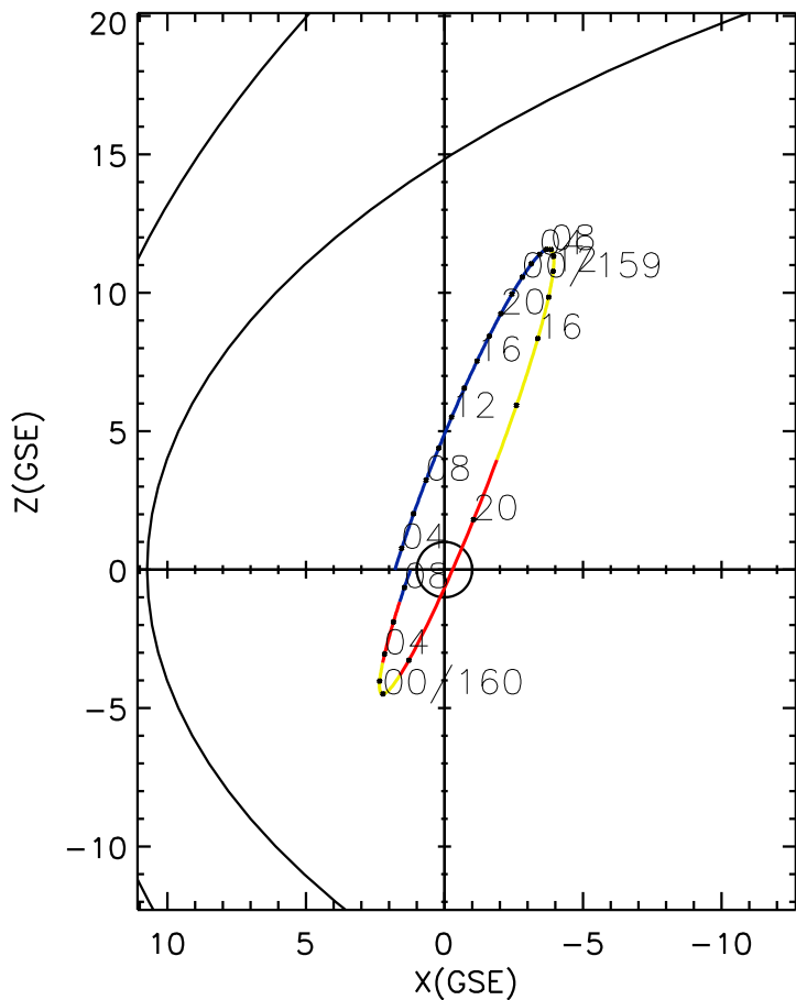
CLUSTER 2 orbit 2022 158 (06/07) 02:46 UT to 2022 160 (06/09) 09:01 UT
