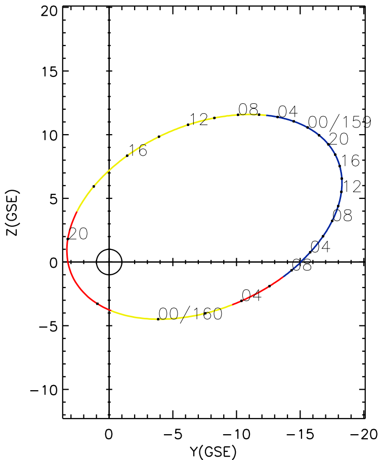
CLUSTER 2 orbit 2022 158 (06/07) 02:46 UT to 2022 160 (06/09) 09:01 UT
