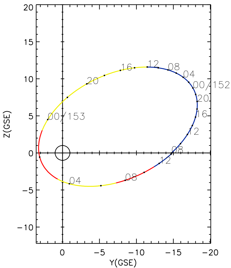
CLUSTER 2 orbit 2022 151 (05/31) 07:56 UT to 2022 153 (06/02) 14:11 UT
