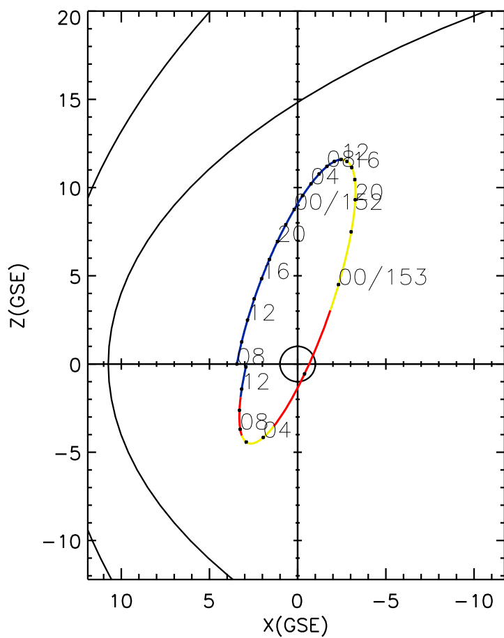
CLUSTER 2 orbit 2022 151 (05/31) 07:56 UT to 2022 153 (06/02) 14:11 UT
