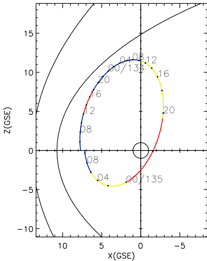
CLUSTER 2 orbit 2022 133 (05/13) 04:16 UT to 2022 135 (05/15) 10:31 UT
