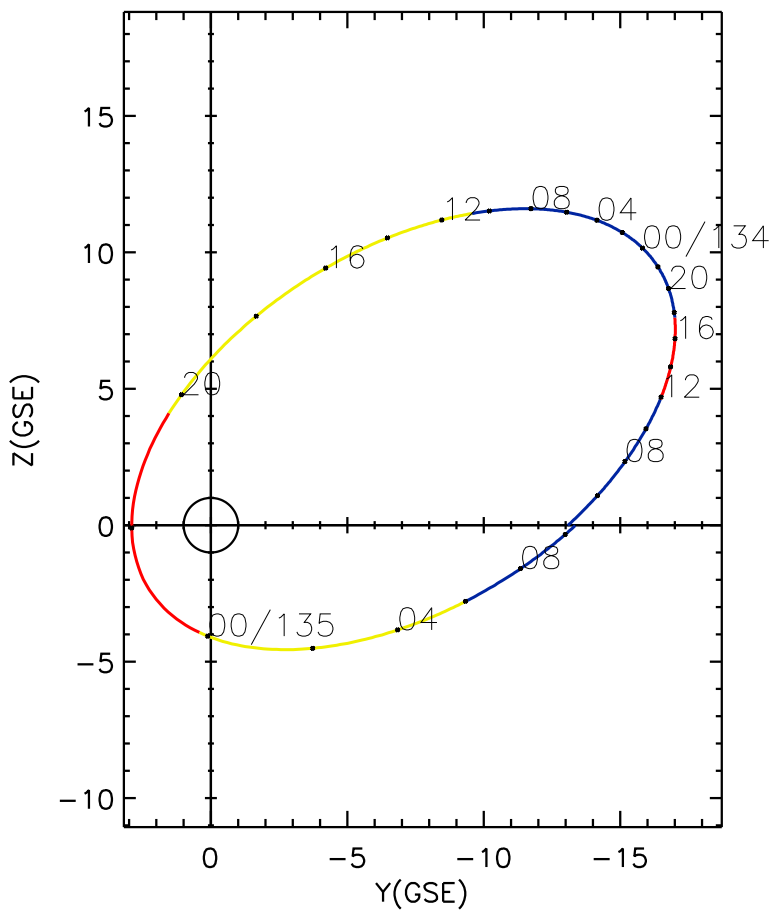
CLUSTER 2 orbit 2022 133 (05/13) 04:16 UT to 2022 135 (05/15) 10:31 UT
