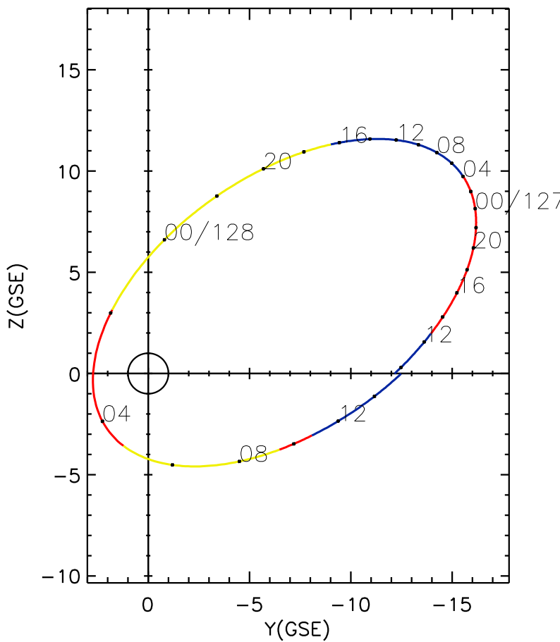
CLUSTER 2 orbit 2022 126 (05/06) 09:31 UT to 2022 128 (05/08) 15:46 UT
