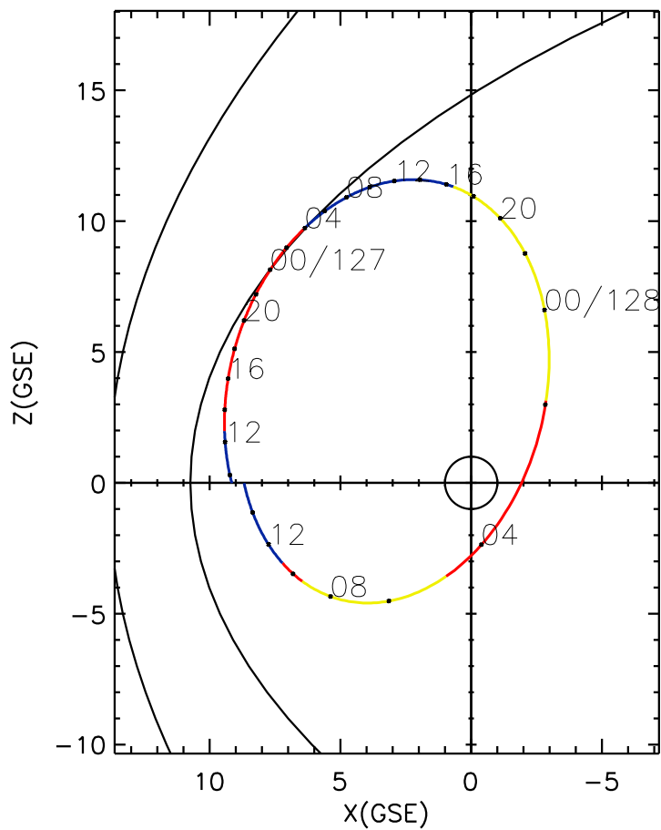
CLUSTER 2 orbit 2022 126 (05/06) 09:31 UT to 2022 128 (05/08) 15:46 UT
