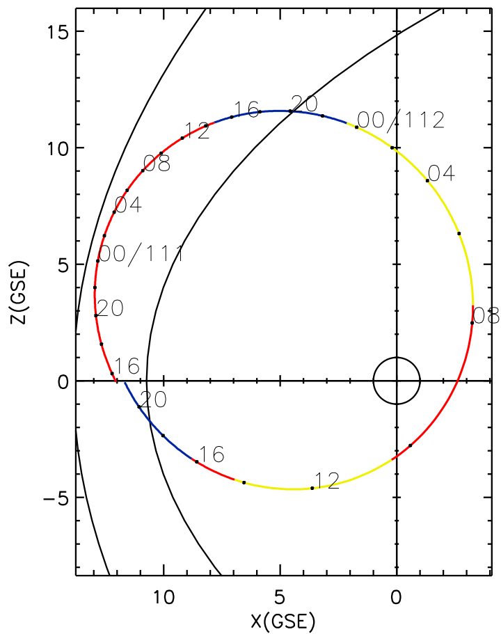
CLUSTER 2 orbit 2022 110 (04/20) 15:26 UT to 2022 112 (04/22) 21:41 UT
