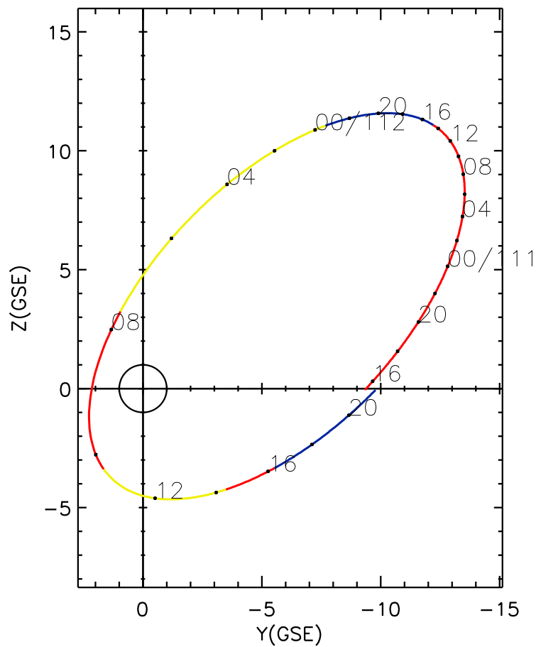
CLUSTER 2 orbit 2022 110 (04/20) 15:26 UT to 2022 112 (04/22) 21:41 UT
