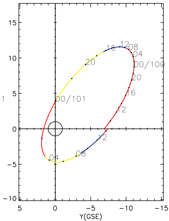
CLUSTER 2 orbit 2022 099 (04/09) 08:11 UT to 2022 101 (04/11) 14:26 UT
