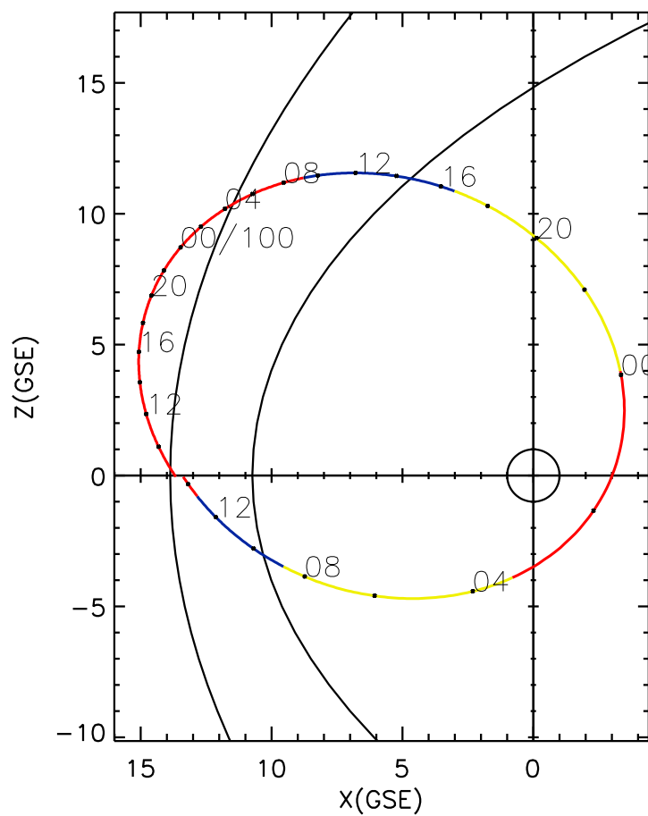
CLUSTER 2 orbit 2022 099 (04/09) 08:11 UT to 2022 101 (04/11) 14:26 UT
