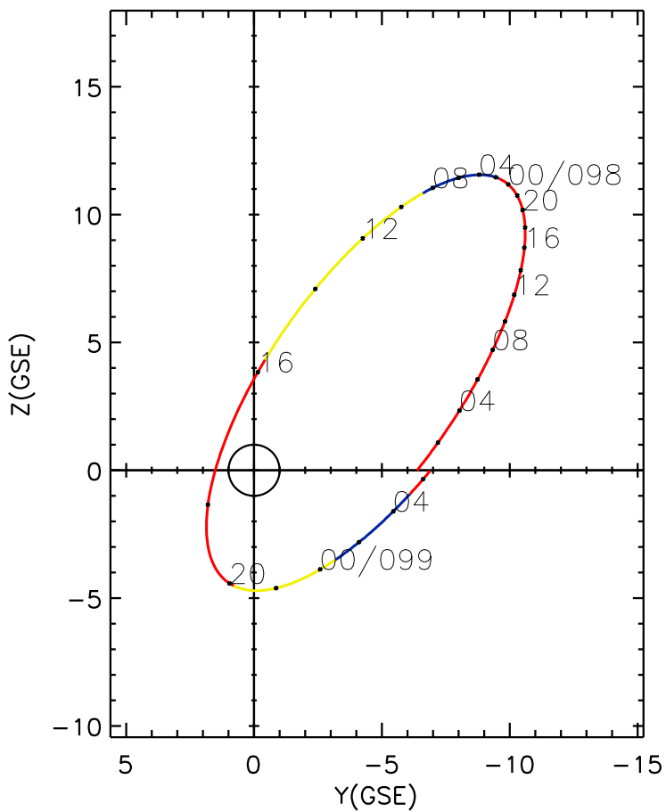
CLUSTER 2 orbit 2022 097 (04/07) 00:16 UT to 2022 099 (04/09) 06:31 UT
