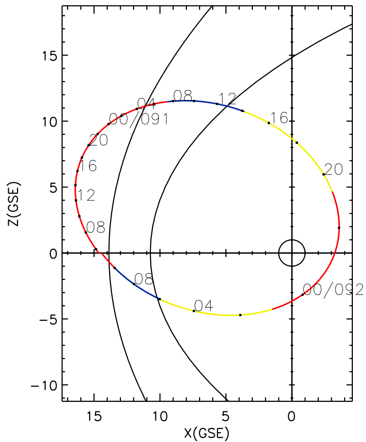
CLUSTER 2 orbit 2022 090 (03/31) 05:31 UT to 2022 092 (04/02) 11:46 UT
